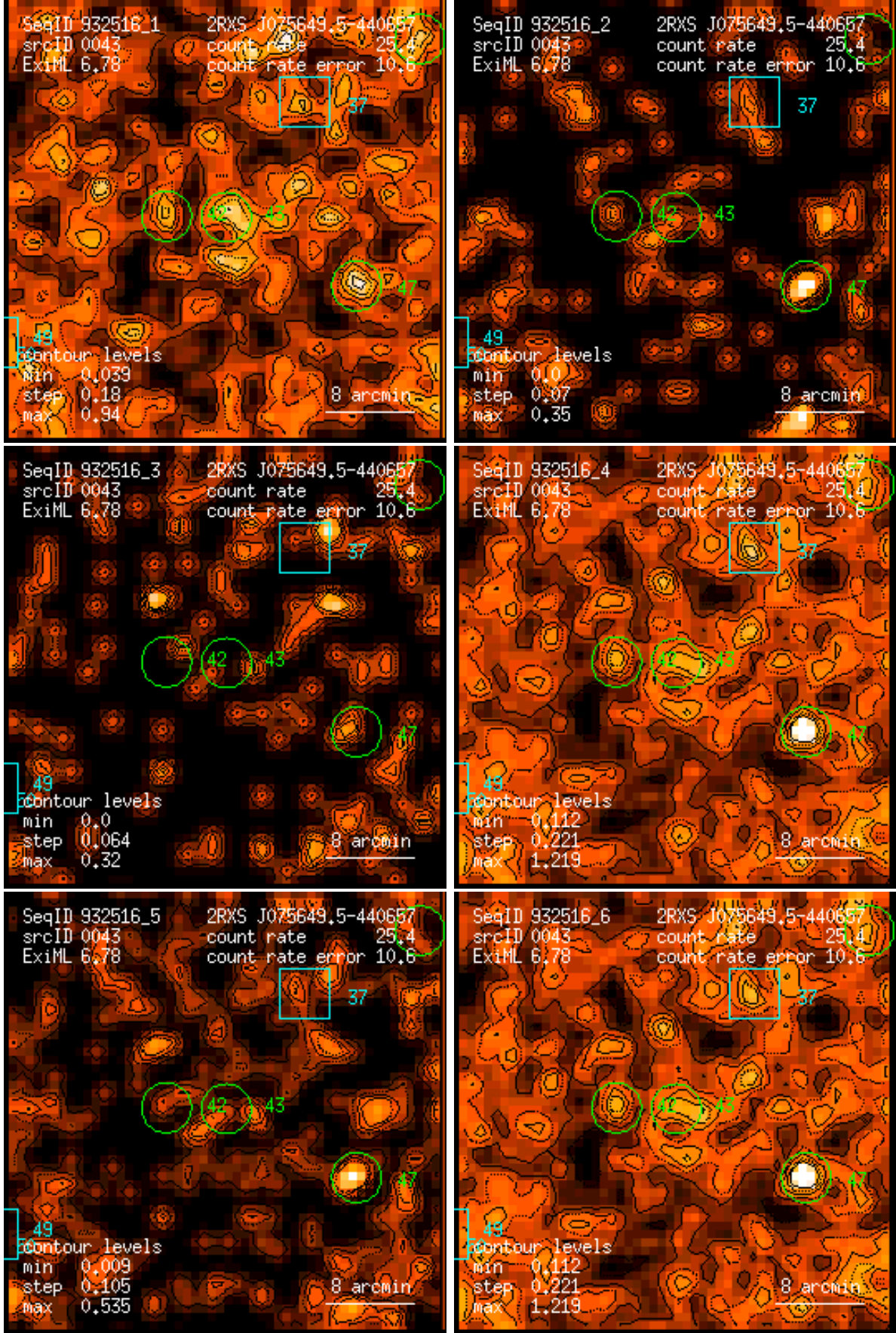
Figure 43: RASS 932516: detection 0043: band rate images, Gaussian filter: (1) PSPC channels 11 – 41, (2) 52 – 90, (3) 91 – 201, (4) 11 – 235, (5) 52 – 201, (6) 11 – 201. Broad band rates in counts/ks. Band rate contour levels in counts/ks/arcmin 2 .
