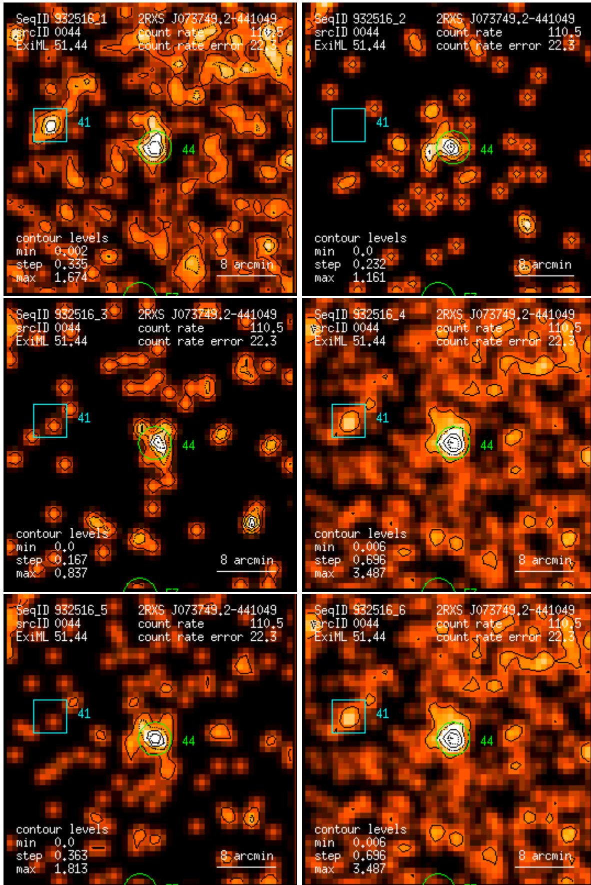
Figure 44: RASS 932516: detection 0044: band rate images, Gaussian filter: (1) PSPC channels 11 – 41, (2) 52 – 90, (3) 91 – 201, (4) 11 – 235, (5) 52 – 201, (6) 11 – 201. Broad band rates in counts/ks. Band rate contour levels in counts/ks/arcmin 2 .
