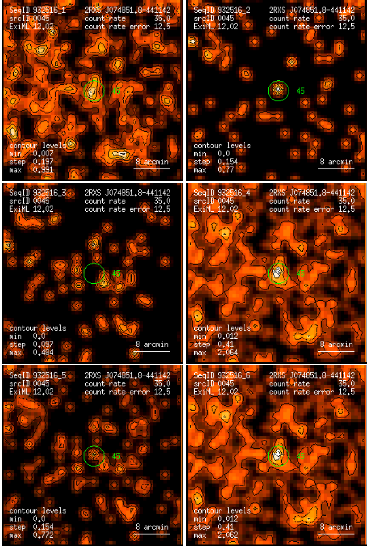
Figure 45: RASS 932516: detection 0045: band rate images, Gaussian filter: (1) PSPC channels 11 – 41, (2) 52 – 90, (3) 91 – 201, (4) 11 – 235, (5) 52 – 201, (6) 11 – 201. Broad band rates in counts/ks. Band rate contour levels in counts/ks/arcmin 2 .
