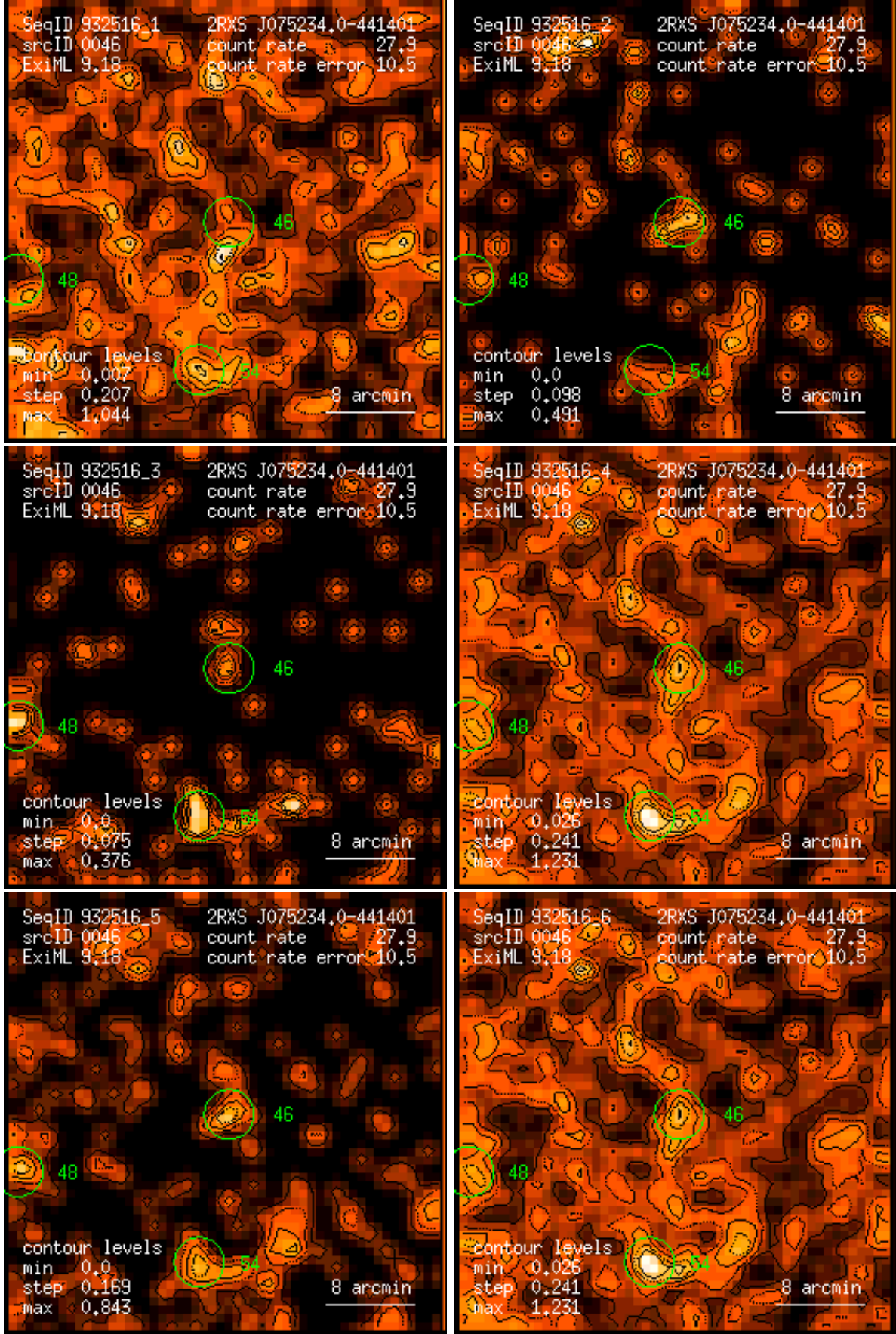
Figure 46: RASS 932516: detection 0046: band rate images, Gaussian filter: (1) PSPC channels 11 – 41, (2) 52 – 90, (3) 91 – 201, (4) 11 – 235, (5) 52 – 201, (6) 11 – 201. Broad band rates in counts/ks. Band rate contour levels in counts/ks/arcmin 2 .
