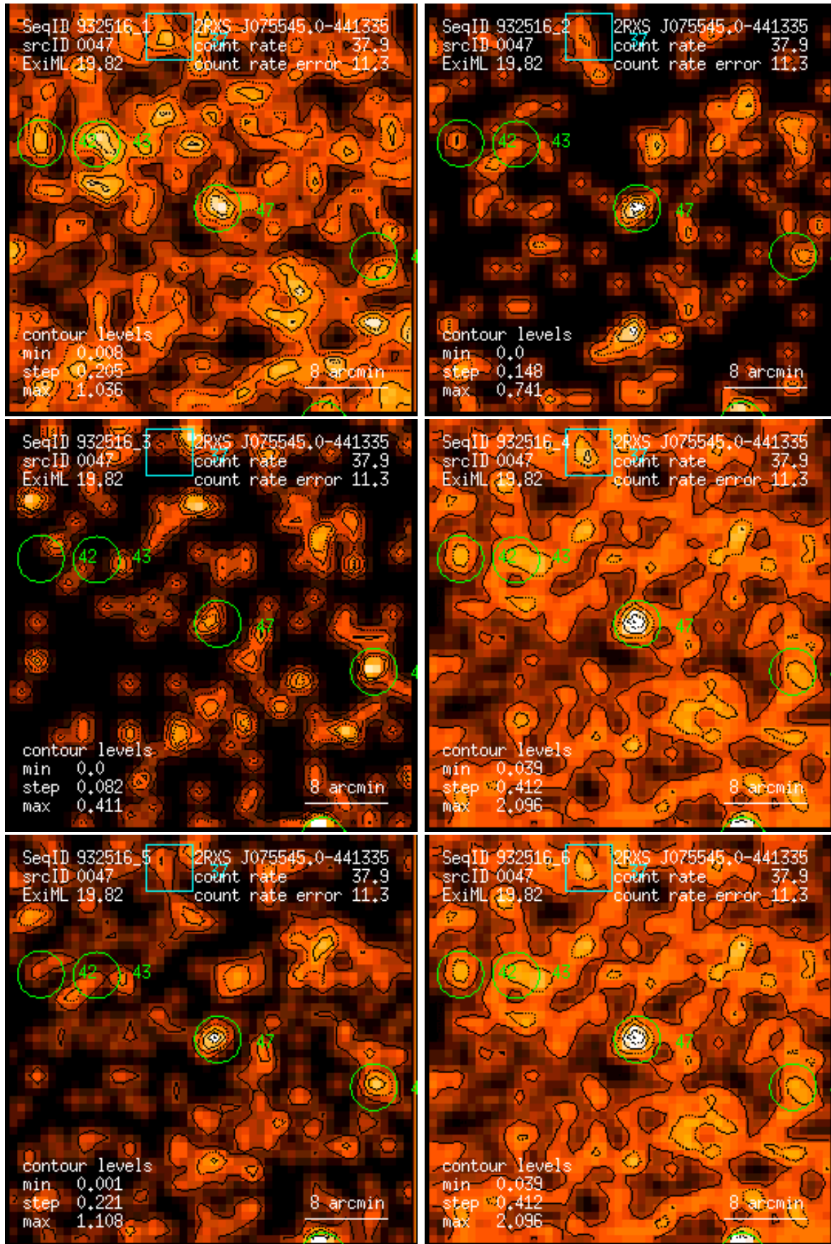
Figure 47: RASS 932516: detection 0047: band rate images, Gaussian filter: (1) PSPC channels 11 – 41, (2) 52 – 90, (3) 91 – 201, (4) 11 – 235, (5) 52 – 201, (6) 11 – 201. Broad band rates in counts/ks. Band rate contour levels in counts/ks/arcmin 2 .
