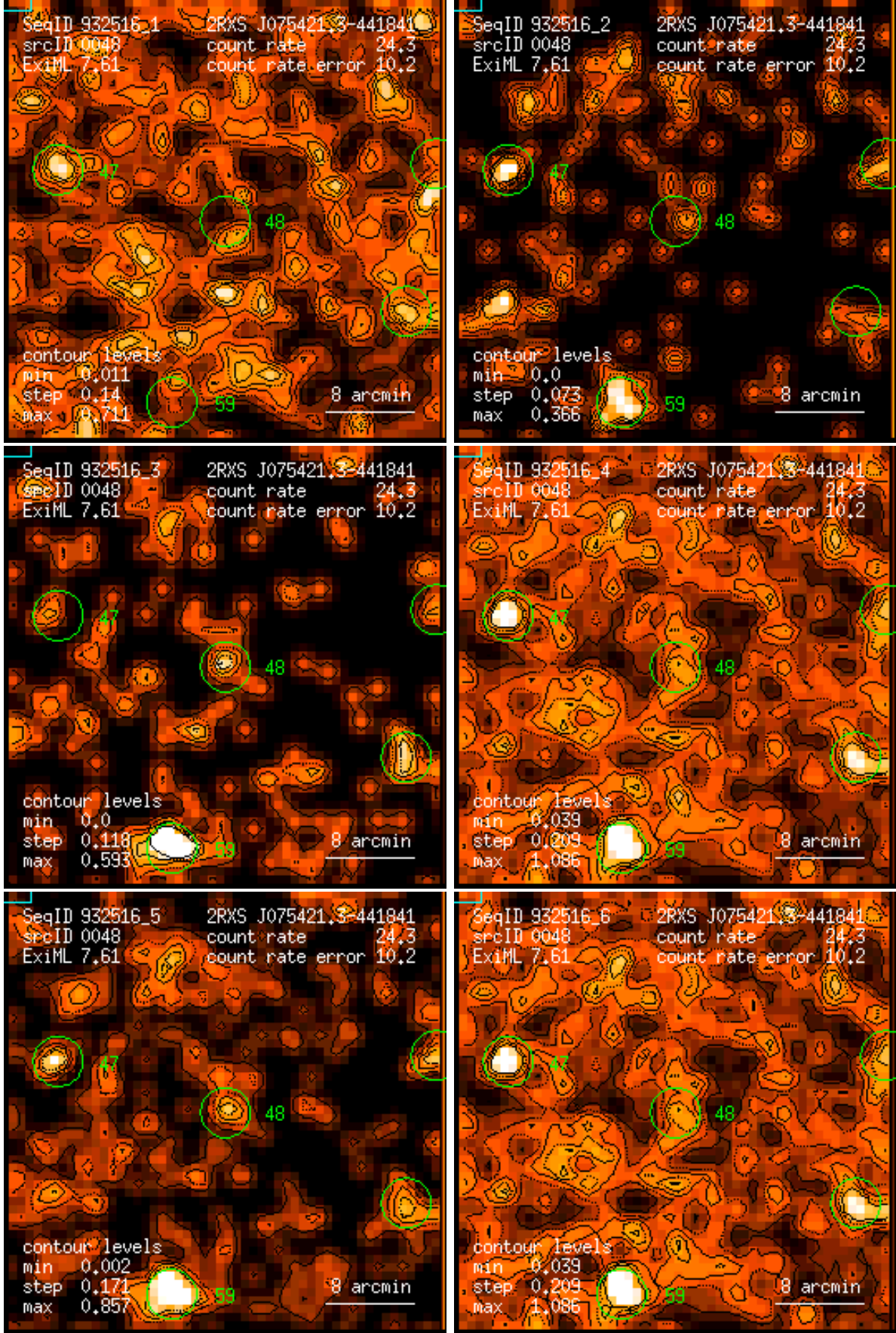
Figure 48: RASS 932516: detection 0048: band rate images, Gaussian filter: (1) PSPC channels 11 – 41, (2) 52 – 90, (3) 91 – 201, (4) 11 – 235, (5) 52 – 201, (6) 11 – 201. Broad band rates in counts/ks. Band rate contour levels in counts/ks/arcmin 2 .
