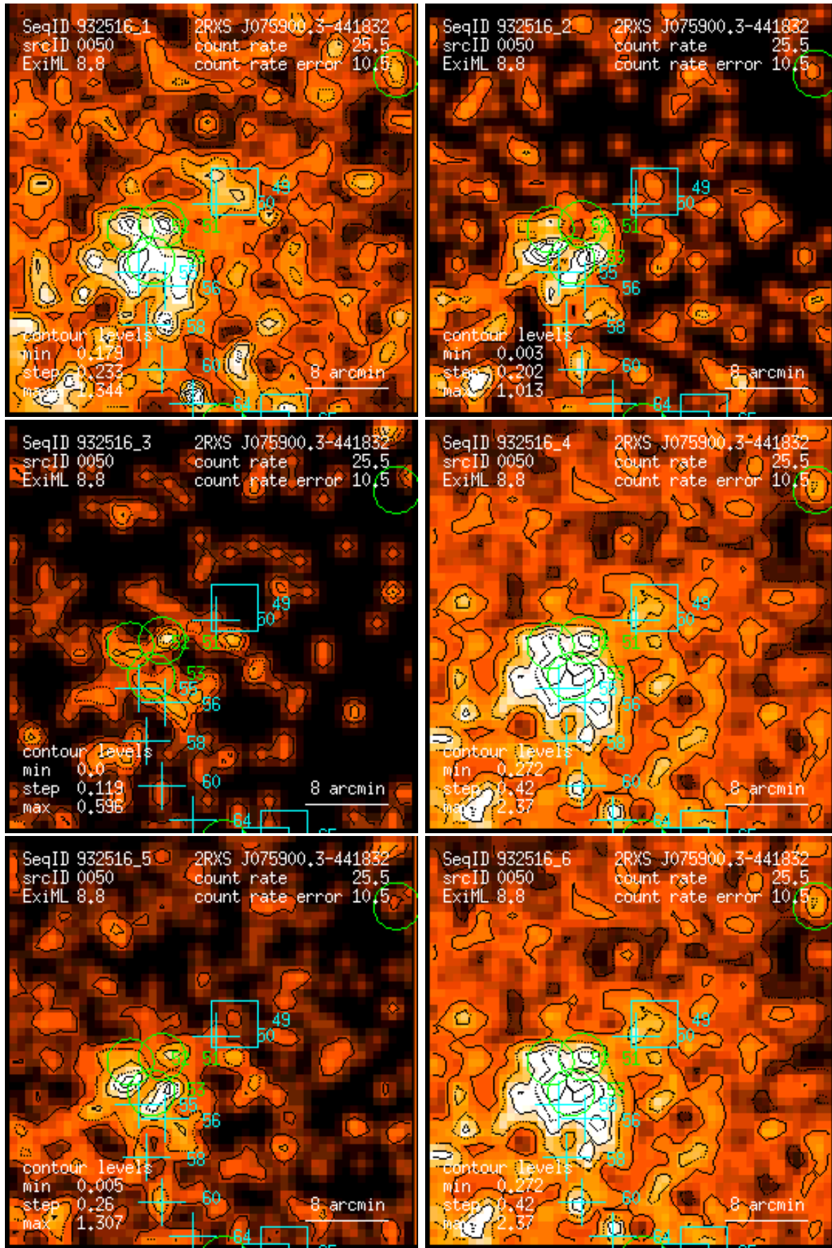
Figure 50: RASS 932516: detection 0050: band rate images, Gaussian filter: (1) PSPC channels 11 – 41, (2) 52 – 90, (3) 91 – 201, (4) 11 – 235, (5) 52 – 201, (6) 11 – 201. Broad band rates in counts/ks. Band rate contour levels in counts/ks/arcmin 2 .
