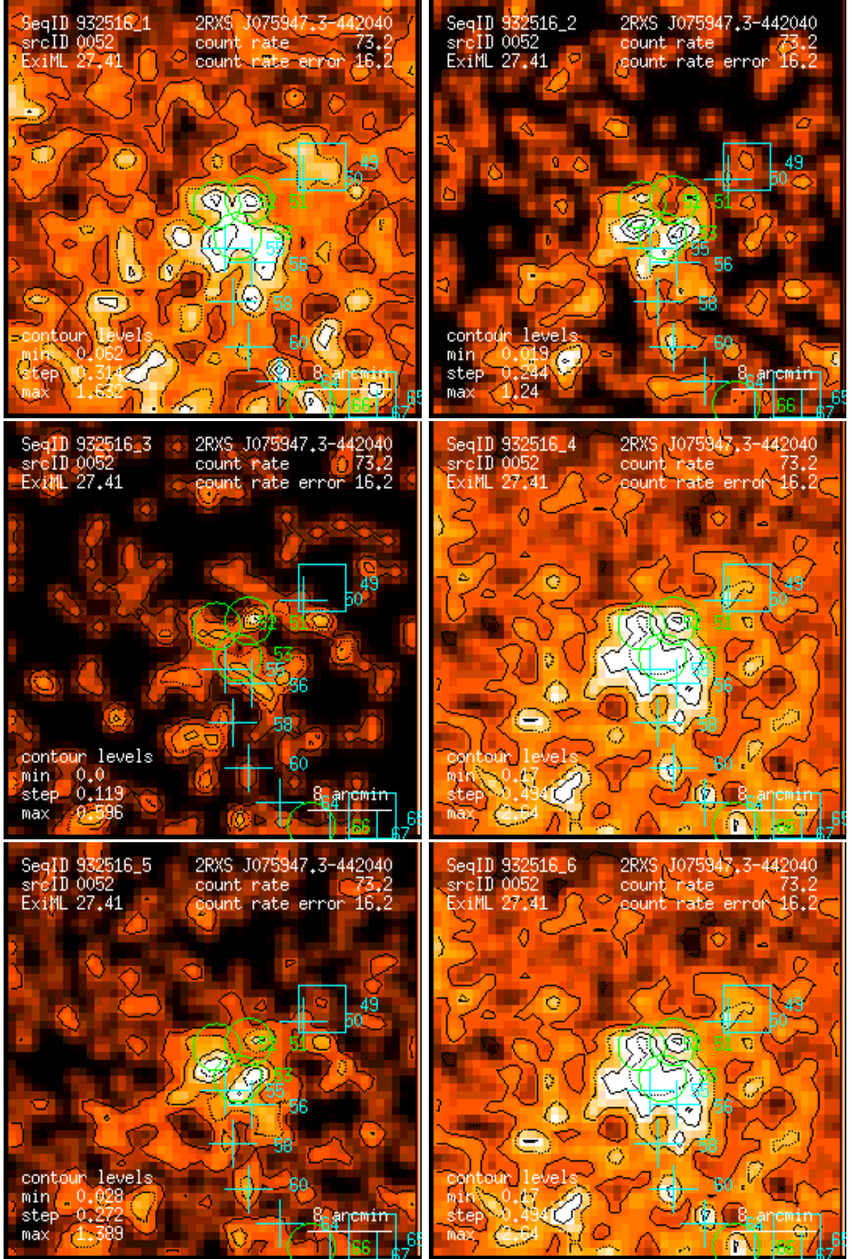
Figure 52: RASS 932516: detection 0052: band rate images, Gaussian filter: (1) PSPC channels 11 – 41, (2) 52 – 90, (3) 91 – 201, (4) 11 – 235, (5) 52 – 201, (6) 11 – 201. Broad band rates in counts/ks. Band rate contour levels in counts/ks/arcmin 2 .
