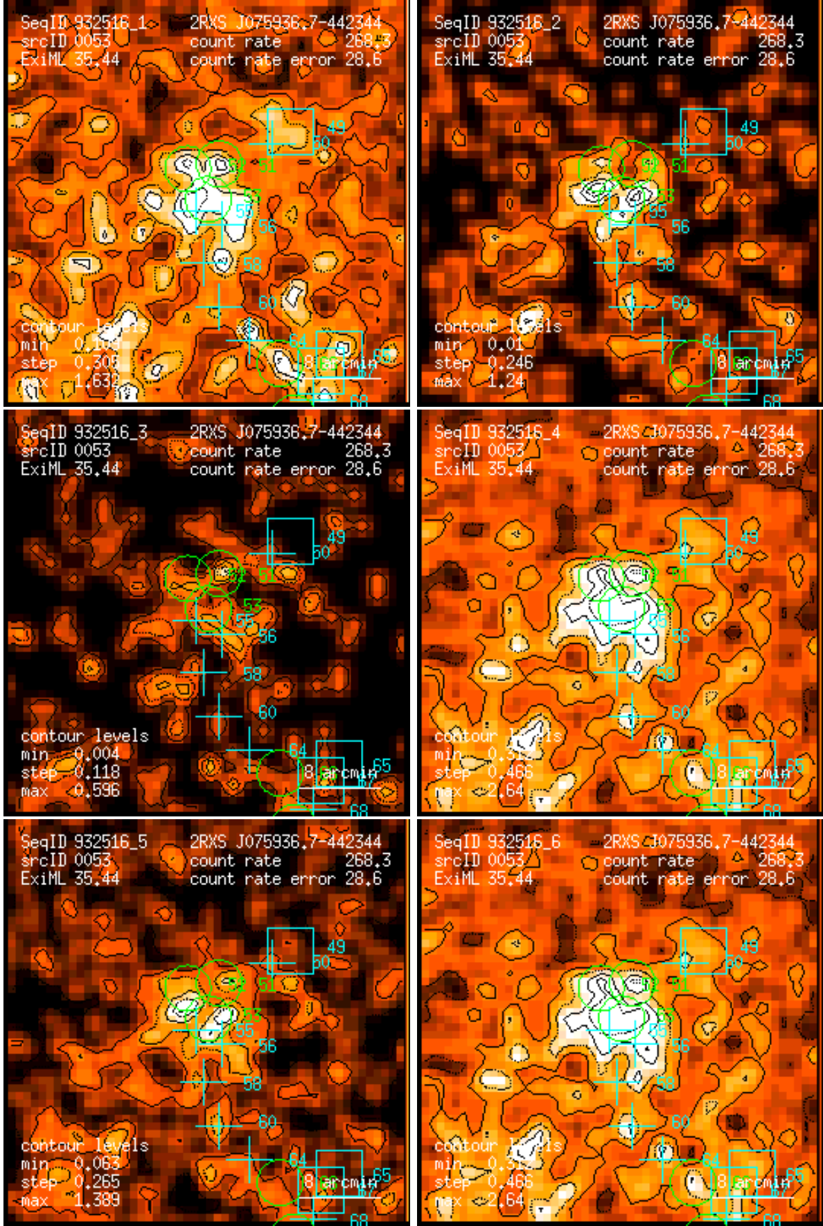
Figure 53: RASS 932516: detection 0053: band rate images, Gaussian filter: (1) PSPC channels 11 – 41, (2) 52 – 90, (3) 91 – 201, (4) 11 – 235, (5) 52 – 201, (6) 11 – 201. Broad band rates in counts/ks. Band rate contour levels in counts/ks/arcmin 2 .
