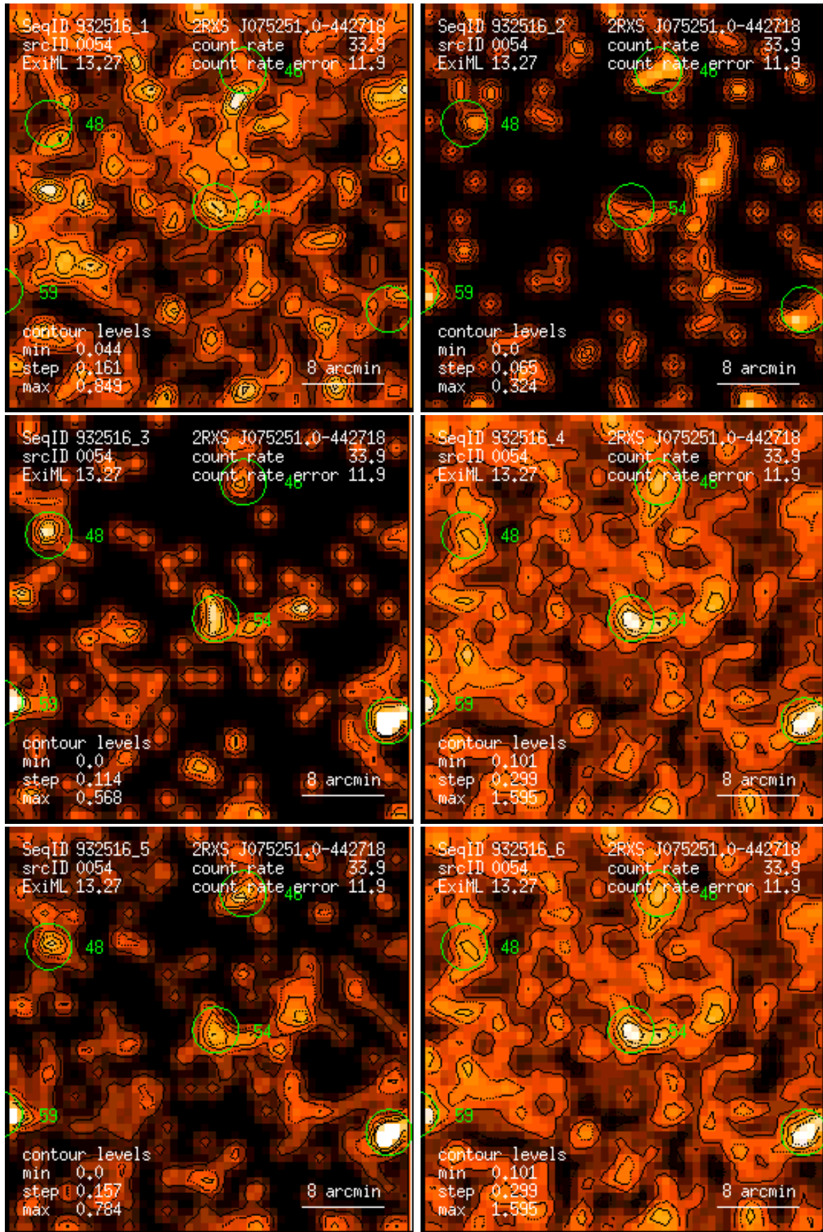
Figure 54: RASS 932516: detection 0054: band rate images, Gaussian filter: (1) PSPC channels 11 – 41, (2) 52 – 90, (3) 91 – 201, (4) 11 – 235, (5) 52 – 201, (6) 11 – 201. Broad band rates in counts/ks. Band rate contour levels in counts/ks/arcmin 2 .
