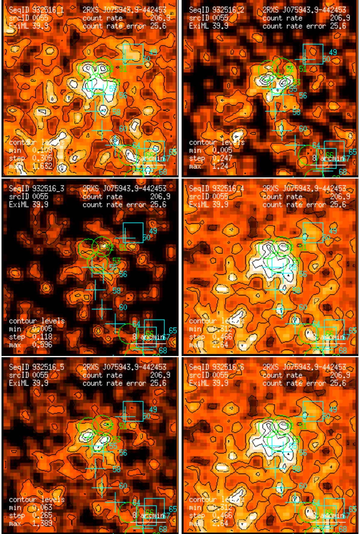
Figure 55: RASS 932516: detection 0055: band rate images, Gaussian filter: (1) PSPC channels 11 – 41, (2) 52 – 90, (3) 91 – 201, (4) 11 – 235, (5) 52 – 201, (6) 11 – 201. Broad band rates in counts/ks. Band rate contour levels in counts/ks/arcmin 2 .
