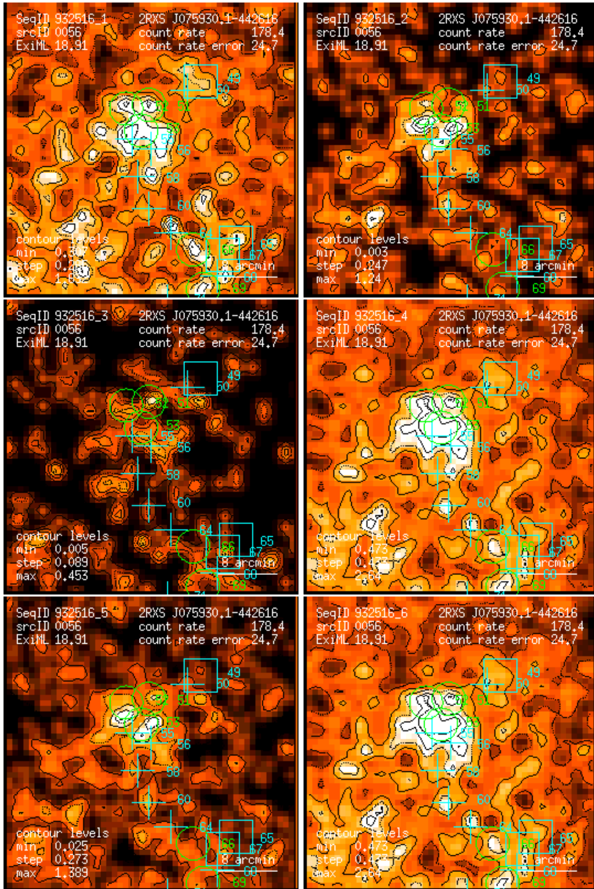
Figure 56: RASS 932516: detection 0056: band rate images, Gaussian filter: (1) PSPC channels 11 – 41, (2) 52 – 90, (3) 91 – 201, (4) 11 – 235, (5) 52 – 201, (6) 11 – 201. Broad band rates in counts/ks. Band rate contour levels in counts/ks/arcmin 2 .
