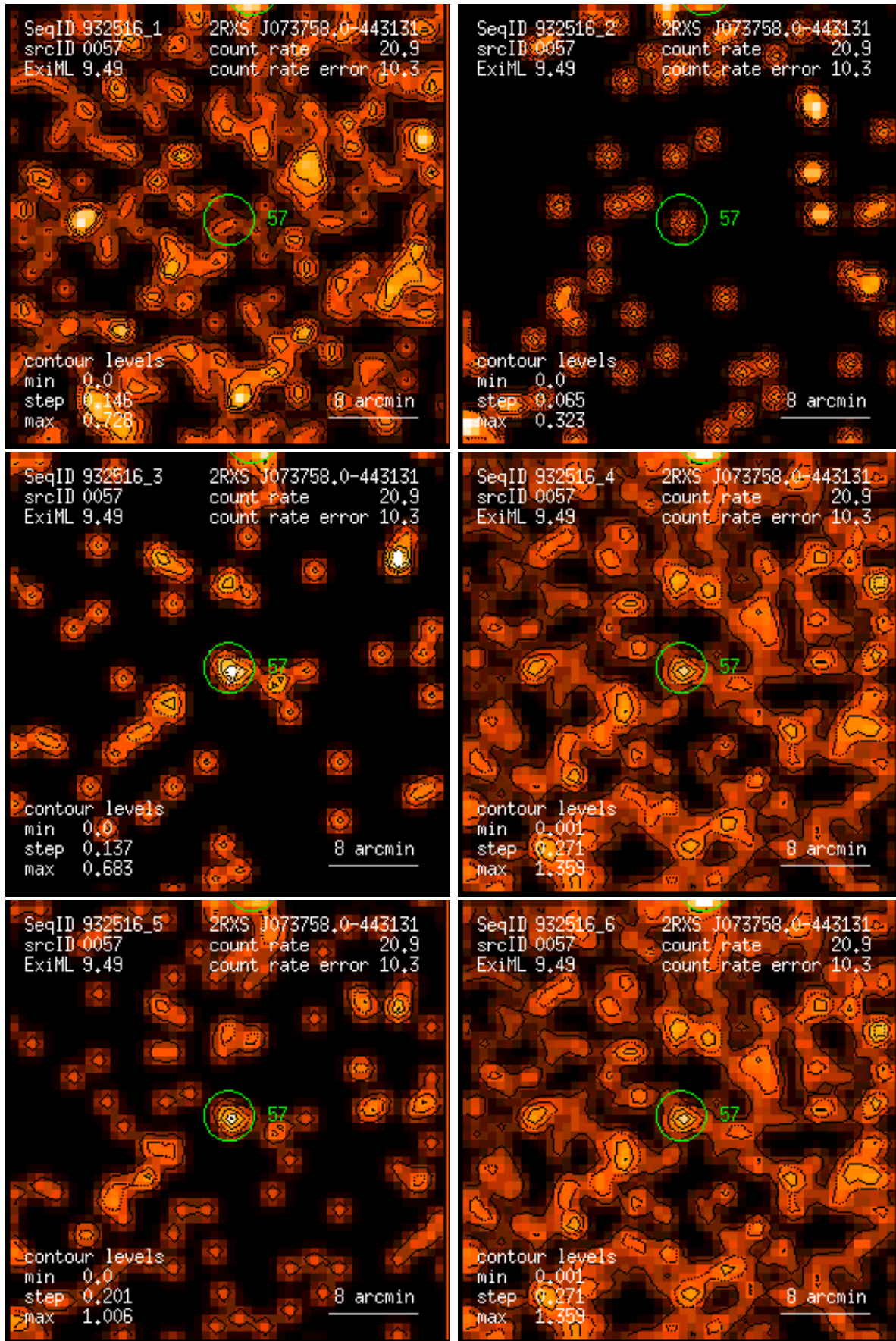
Figure 57: RASS 932516: detection 0057: band rate images, Gaussian filter: (1) PSPC channels 11 – 41, (2) 52 – 90, (3) 91 – 201, (4) 11 – 235, (5) 52 – 201, (6) 11 – 201. Broad band rates in counts/ks. Band rate contour levels in counts/ks/arcmin 2 .
