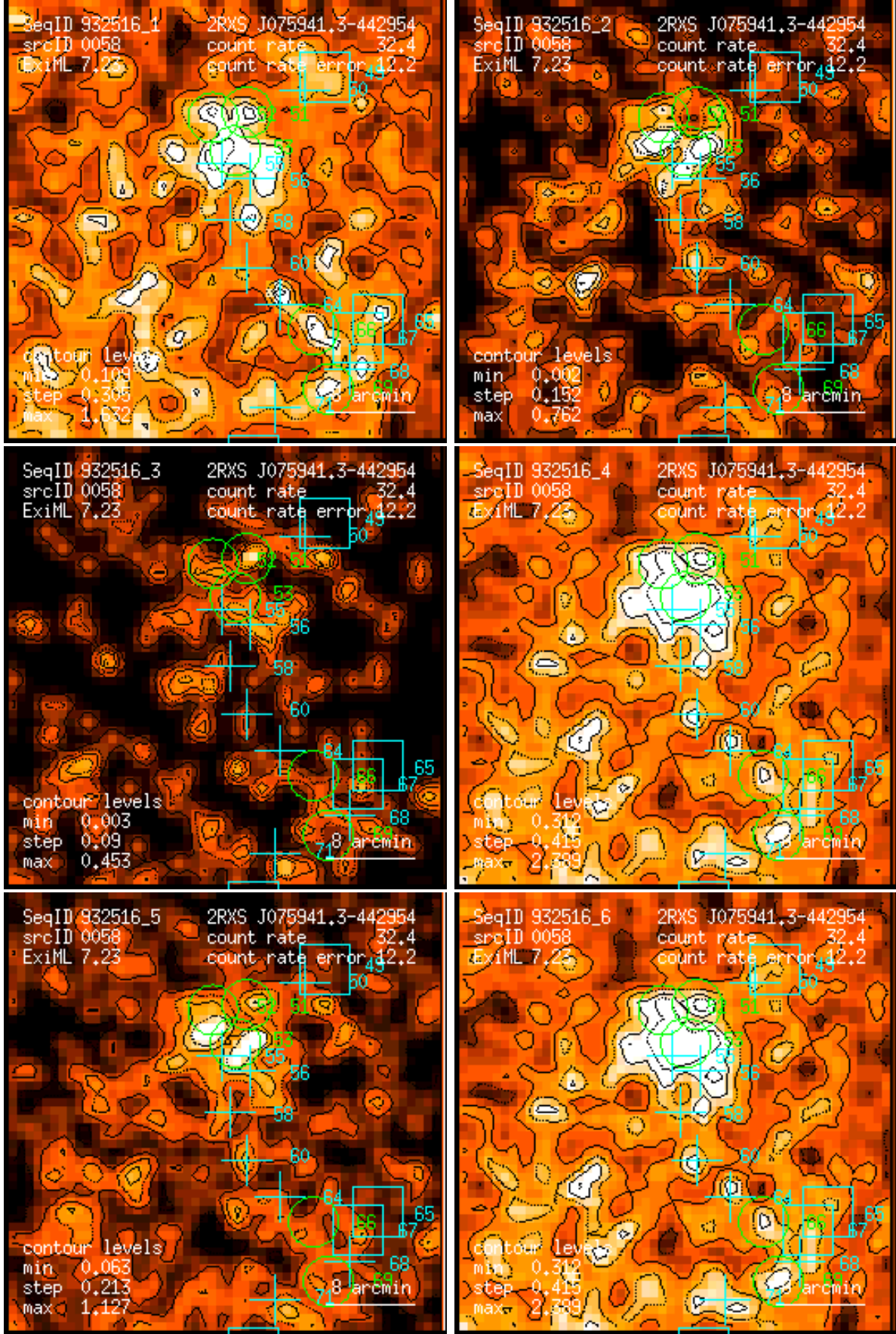
Figure 58: RASS 932516: detection 0058: band rate images, Gaussian filter: (1) PSPC channels 11 – 41, (2) 52 – 90, (3) 91 – 201, (4) 11 – 235, (5) 52 – 201, (6) 11 – 201. Broad band rates in counts/ks. Band rate contour levels in counts/ks/arcmin 2 .
