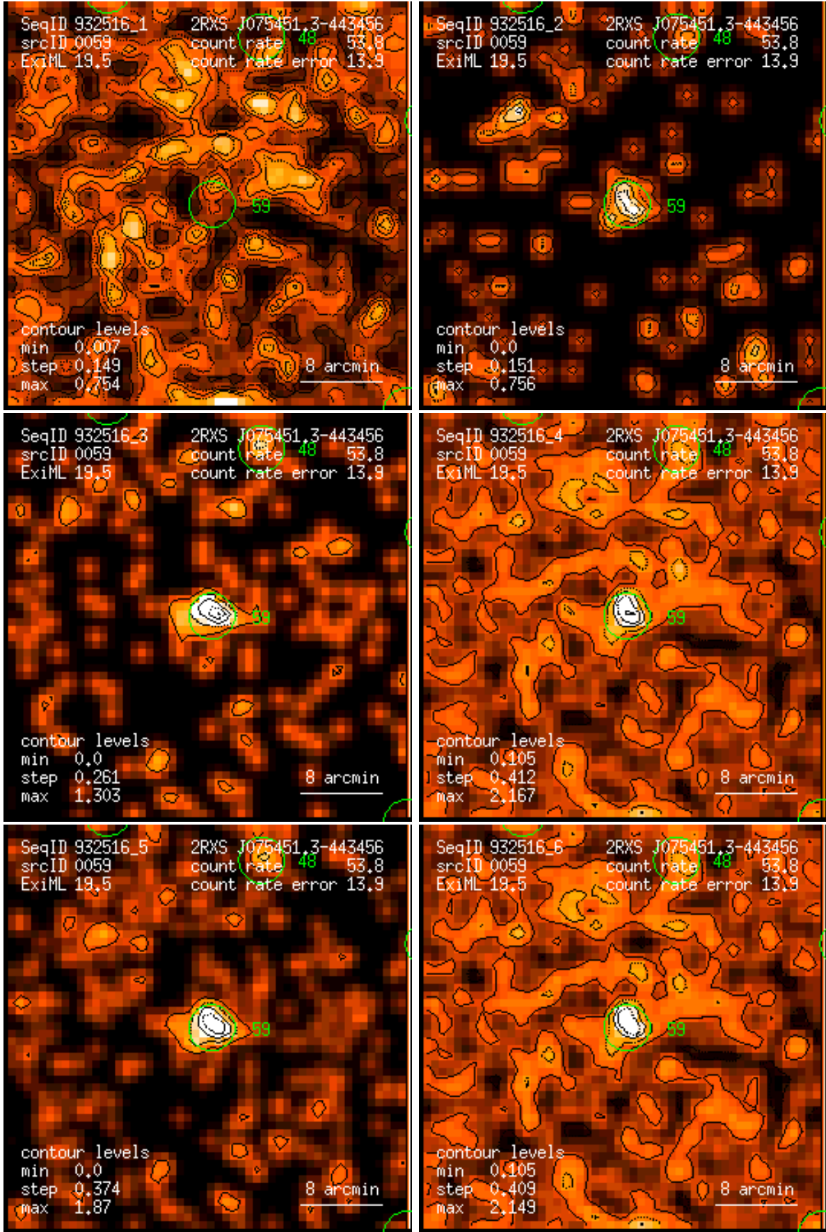
Figure 59: RASS 932516: detection 0059: band rate images, Gaussian filter: (1) PSPC channels 11 – 41, (2) 52 – 90, (3) 91 – 201, (4) 11 – 235, (5) 52 – 201, (6) 11 – 201. Broad band rates in counts/ks. Band rate contour levels in counts/ks/arcmin 2 .
