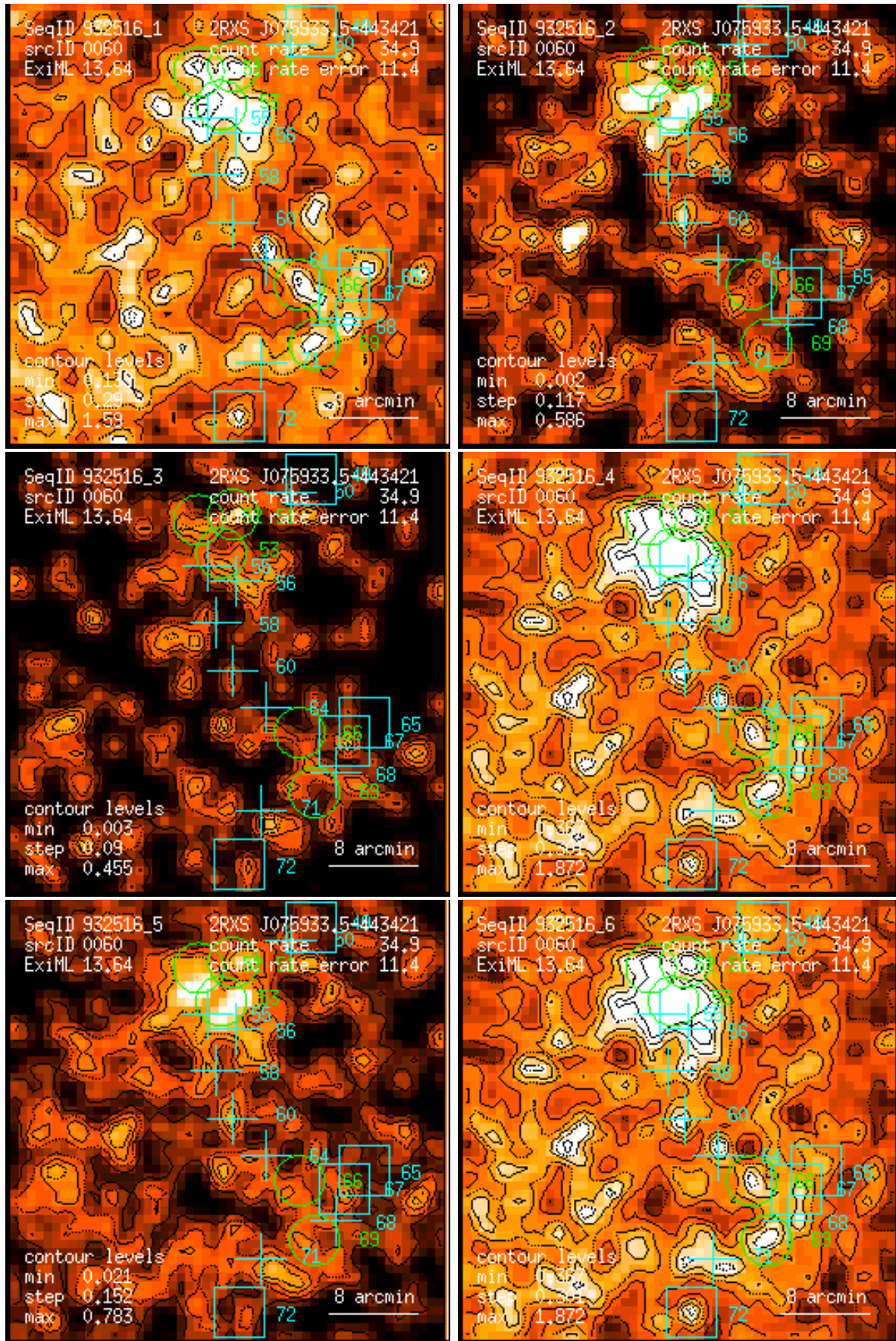
Figure 60: RASS 932516: detection 0060: band rate images, Gaussian filter: (1) PSPC channels 11 – 41, (2) 52 – 90, (3) 91 – 201, (4) 11 – 235, (5) 52 – 201, (6) 11 – 201. Broad band rates in counts/ks. Band rate contour levels in counts/ks/arcmin 2 .
