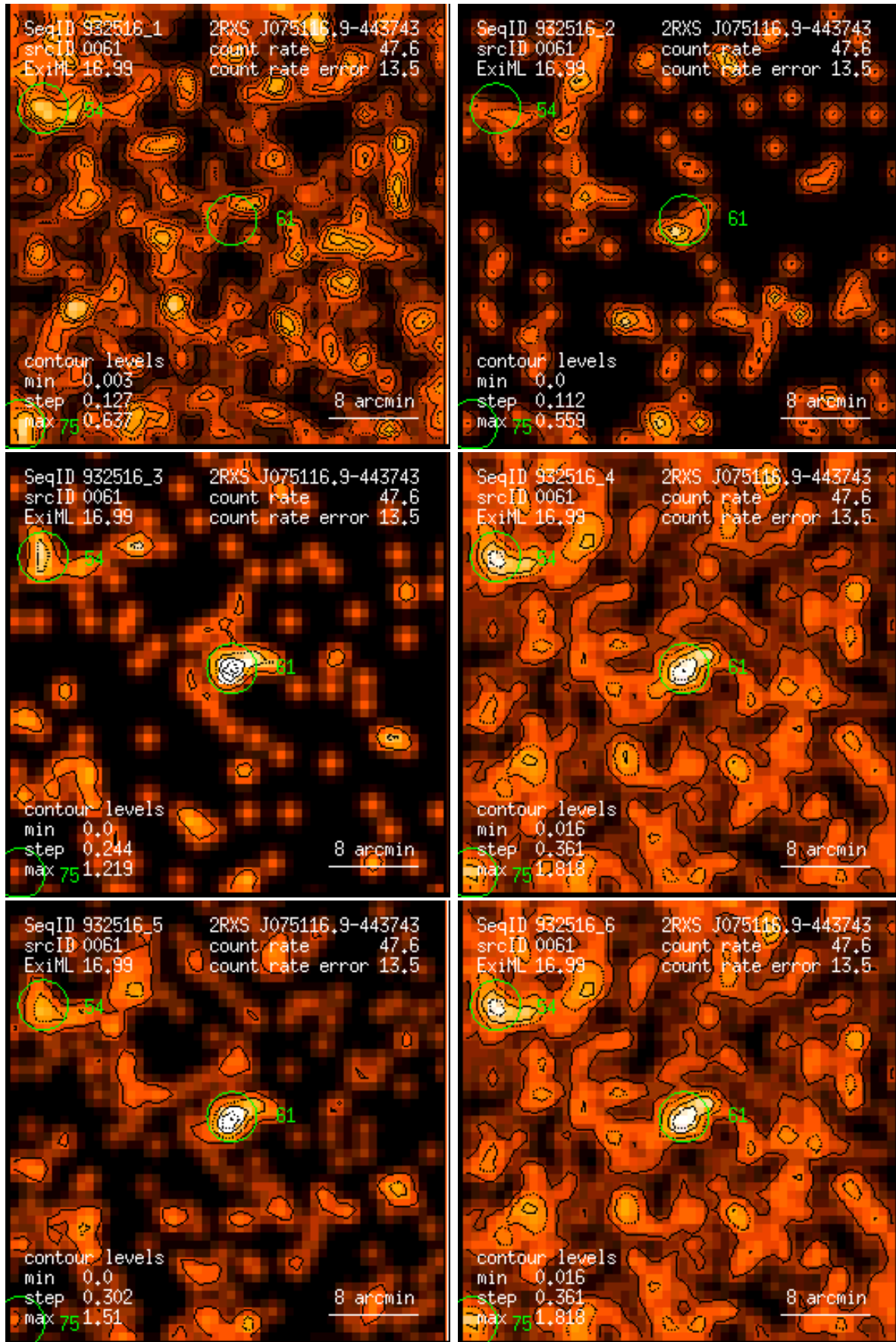
Figure 61: RASS 932516: detection 0061: band rate images, Gaussian filter: (1) PSPC channels 11 – 41, (2) 52 – 90, (3) 91 – 201, (4) 11 – 235, (5) 52 – 201, (6) 11 – 201. Broad band rates in counts/ks. Band rate contour levels in counts/ks/arcmin 2 .
