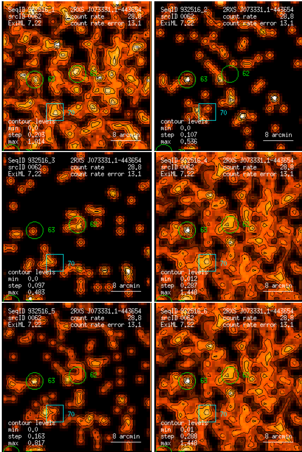
Figure 62: RASS 932516: detection 0062: band rate images, Gaussian filter: (1) PSPC channels 11 – 41, (2) 52 – 90, (3) 91 – 201, (4) 11 – 235, (5) 52 – 201, (6) 11 – 201. Broad band rates in counts/ks. Band rate contour levels in counts/ks/arcmin 2 .
