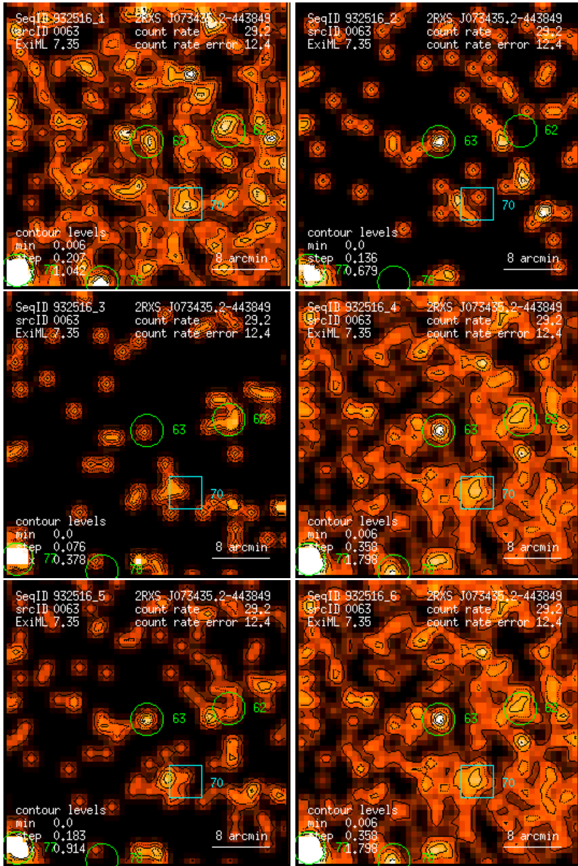
Figure 63: RASS 932516: detection 0063: band rate images, Gaussian filter: (1) PSPC channels 11 – 41, (2) 52 – 90, (3) 91 – 201, (4) 11 – 235, (5) 52 – 201, (6) 11 – 201. Broad band rates in counts/ks. Band rate contour levels in counts/ks/arcmin 2 .
