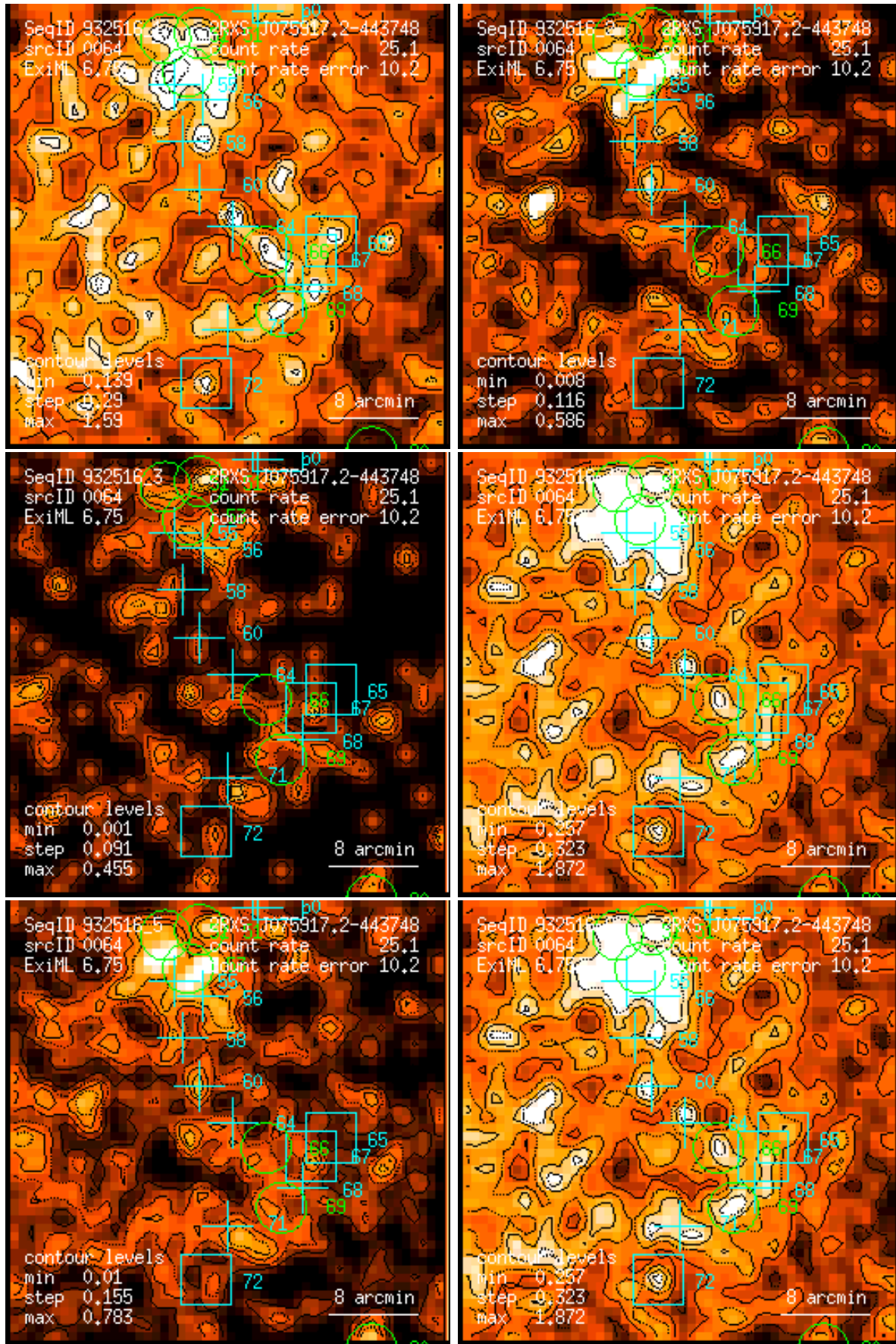
Figure 64: RASS 932516: detection 0064: band rate images, Gaussian filter: (1) PSPC channels 11 – 41, (2) 52 – 90, (3) 91 – 201, (4) 11 – 235, (5) 52 – 201, (6) 11 – 201. Broad band rates in counts/ks. Band rate contour levels in counts/ks/arcmin 2 .
