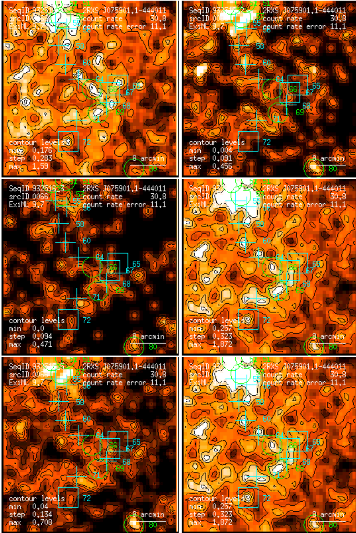
Figure 66: RASS 932516: detection 0066: band rate images, Gaussian filter: (1) PSPC channels 11 – 41, (2) 52 – 90, (3) 91 – 201, (4) 11 – 235, (5) 52 – 201, (6) 11 – 201. Broad band rates in counts/ks. Band rate contour levels in counts/ks/arcmin 2 .
