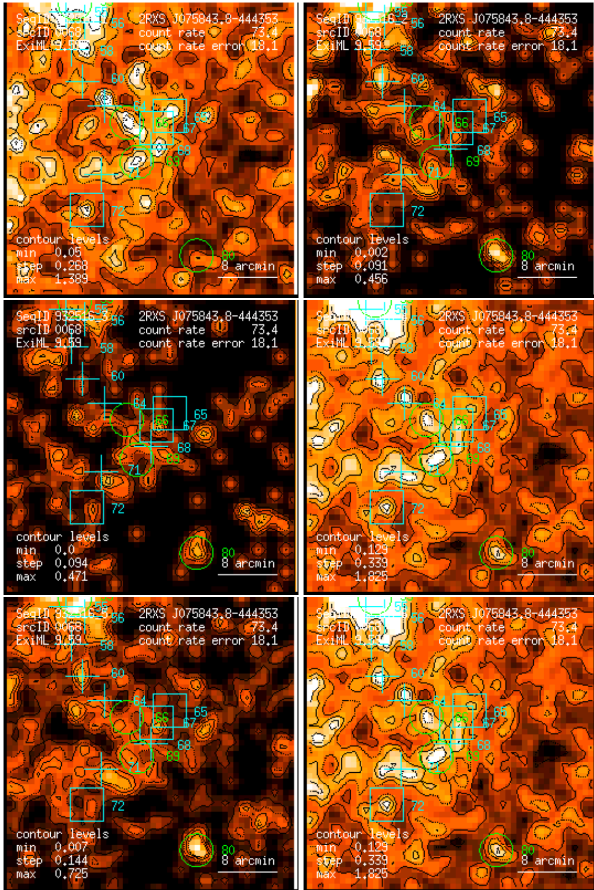
Figure 68: RASS 932516: detection 0068: band rate images, Gaussian filter: (1) PSPC channels 11 – 41, (2) 52 – 90, (3) 91 – 201, (4) 11 – 235, (5) 52 – 201, (6) 11 – 201. Broad band rates in counts/ks. Band rate contour levels in counts/ks/arcmin 2 .
