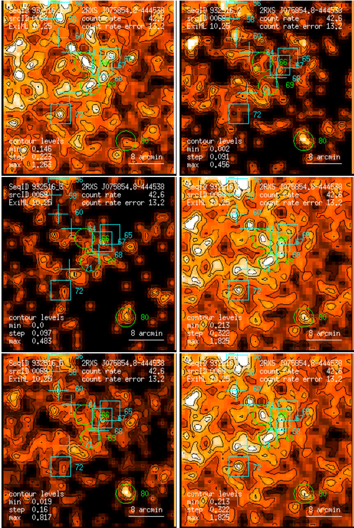
Figure 69: RASS 932516: detection 0069: band rate images, Gaussian filter: (1) PSPC channels 11 – 41, (2) 52 – 90, (3) 91 – 201, (4) 11 – 235, (5) 52 – 201, (6) 11 – 201. Broad band rates in counts/ks. Band rate contour levels in counts/ks/arcmin 2 .
