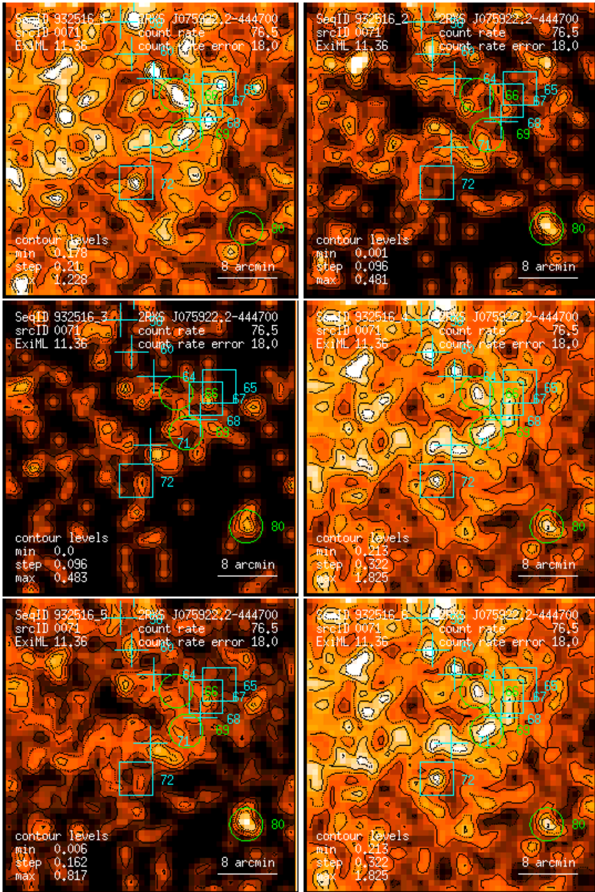
Figure 71: RASS 932516: detection 0071: band rate images, Gaussian filter: (1) PSPC channels 11 – 41, (2) 52 – 90, (3) 91 – 201, (4) 11 – 235, (5) 52 – 201, (6) 11 – 201. Broad band rates in counts/ks. Band rate contour levels in counts/ks/arcmin 2 .
