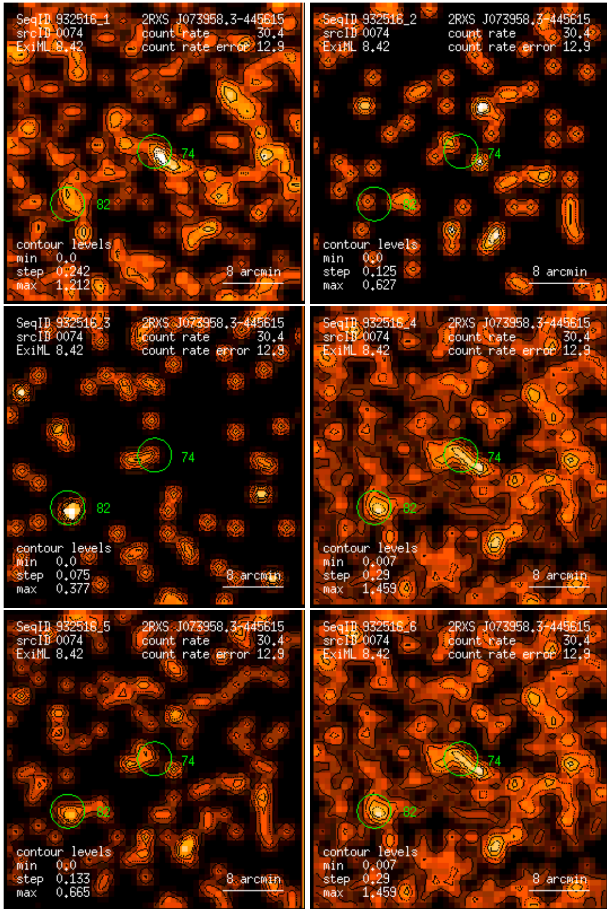
Figure 74: RASS 932516: detection 0074: band rate images, Gaussian filter: (1) PSPC channels 11 – 41, (2) 52 – 90, (3) 91 – 201, (4) 11 – 235, (5) 52 – 201, (6) 11 – 201. Broad band rates in counts/ks. Band rate contour levels in counts/ks/arcmin 2 .
