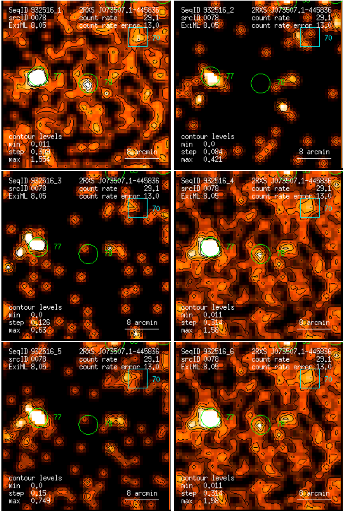
Figure 78: RASS 932516: detection 0078: band rate images, Gaussian filter: (1) PSPC channels 11 – 41, (2) 52 – 90, (3) 91 – 201, (4) 11 – 235, (5) 52 – 201, (6) 11 – 201. Broad band rates in counts/ks. Band rate contour levels in counts/ks/arcmin 2 .
