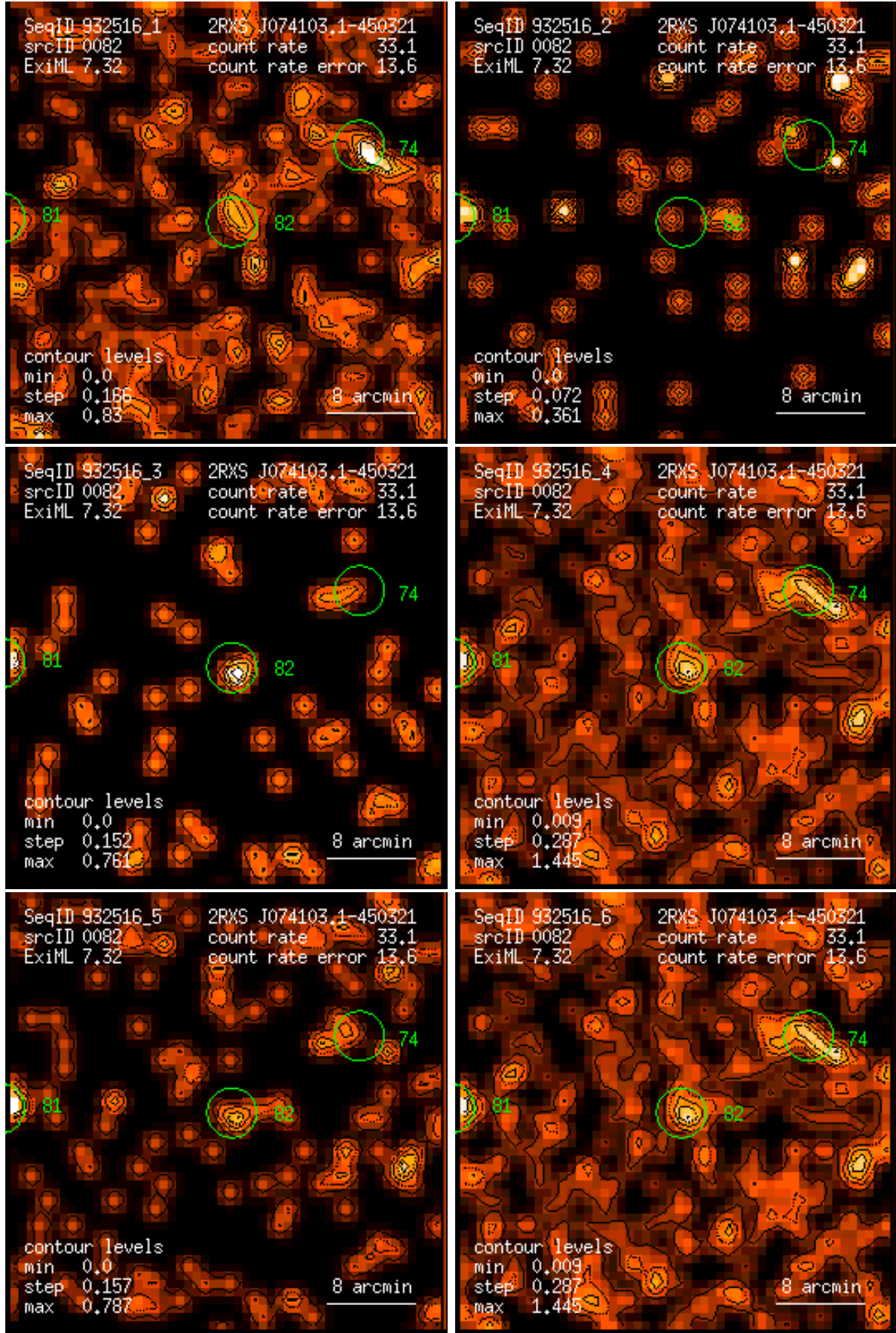
Figure 82: RASS 932516: detection 0082: band rate images, Gaussian filter: (1) PSPC channels 11 – 41, (2) 52 – 90, (3) 91 – 201, (4) 11 – 235, (5) 52 – 201, (6) 11 – 201. Broad band rates in counts/ks. Band rate contour levels in counts/ks/arcmin 2 .
