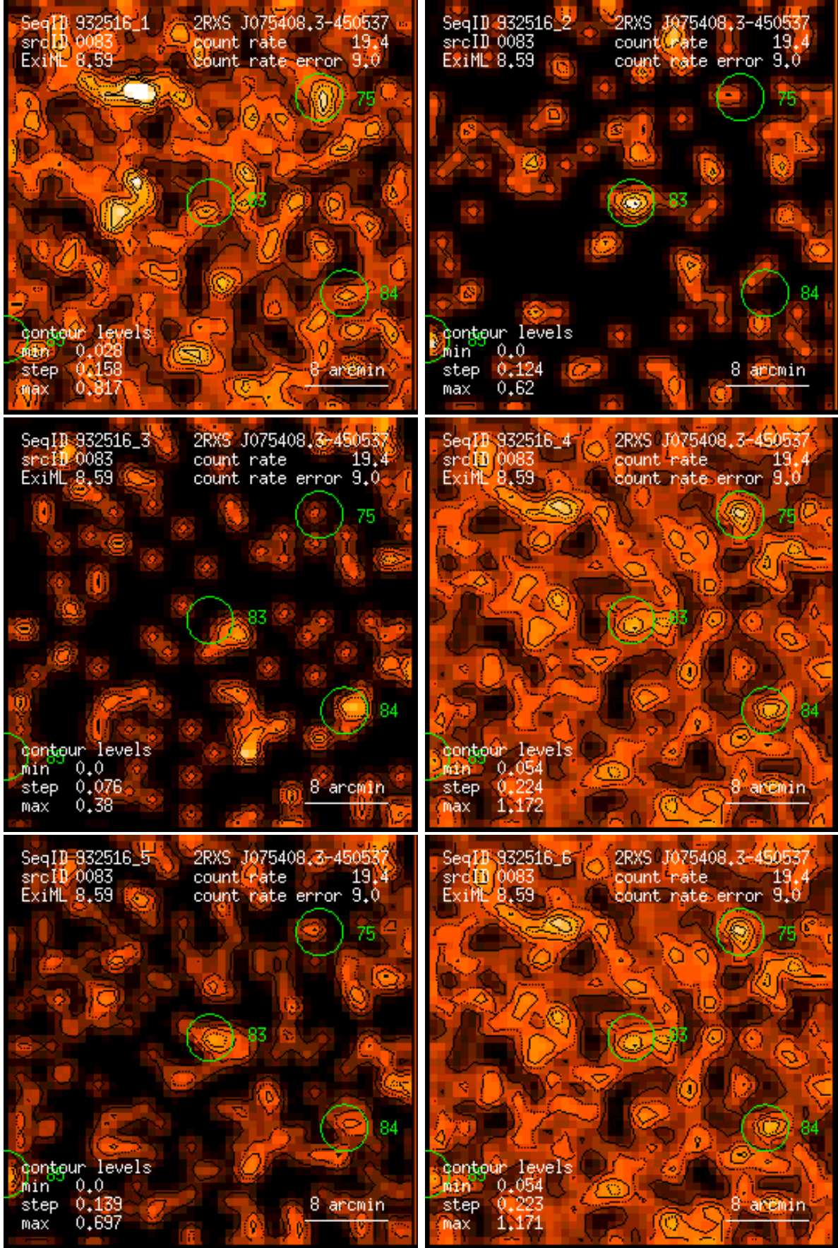
Figure 83: RASS 932516: detection 0083: band rate images, Gaussian filter: (1) PSPC channels 11 – 41, (2) 52 – 90, (3) 91 – 201, (4) 11 – 235, (5) 52 – 201, (6) 11 – 201. Broad band rates in counts/ks. Band rate contour levels in counts/ks/arcmin 2 .
