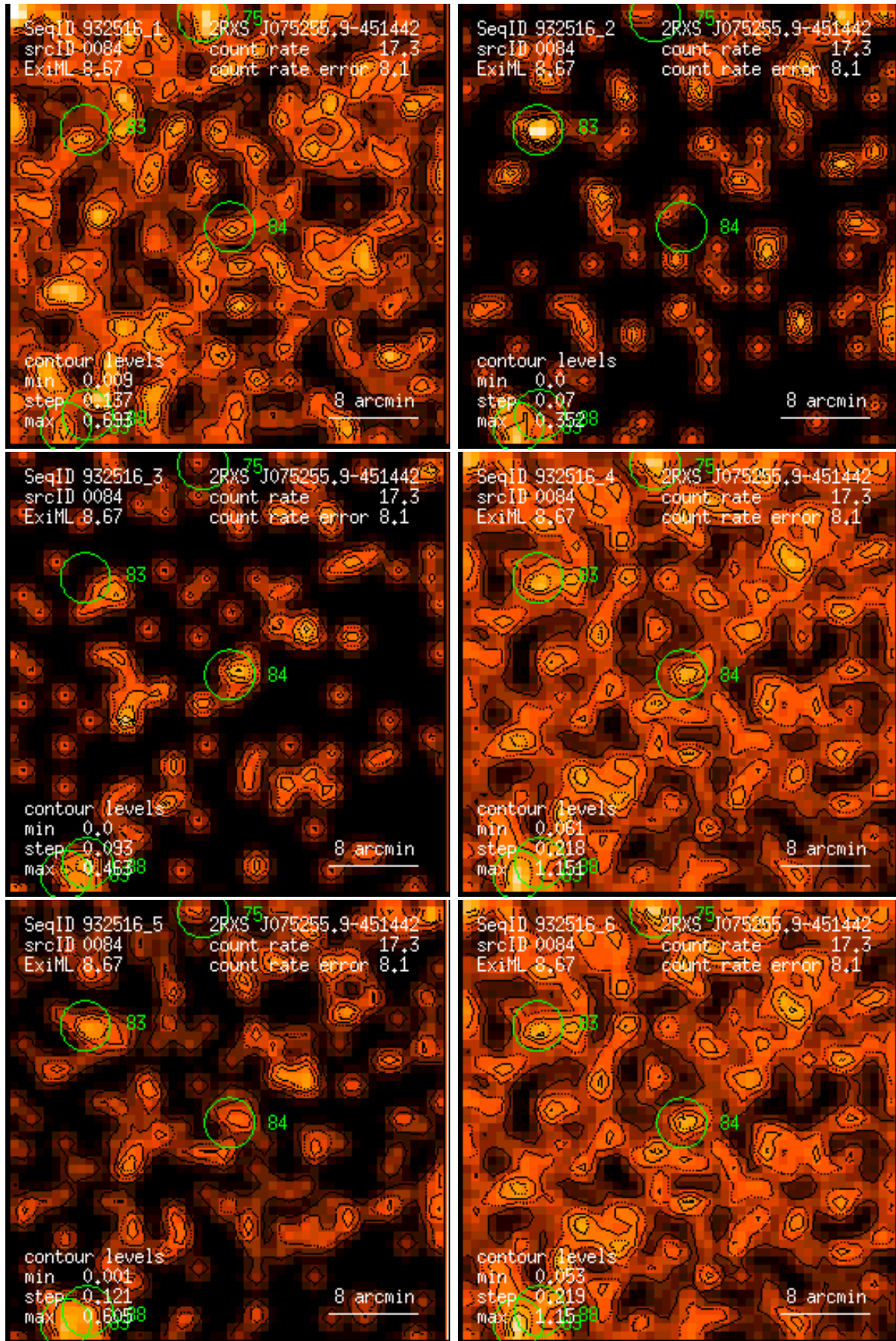
Figure 84: RASS 932516: detection 0084: band rate images, Gaussian filter: (1) PSPC channels 11 – 41, (2) 52 – 90, (3) 91 – 201, (4) 11 – 235, (5) 52 – 201, (6) 11 – 201. Broad band rates in counts/ks. Band rate contour levels in counts/ks/arcmin 2 .
