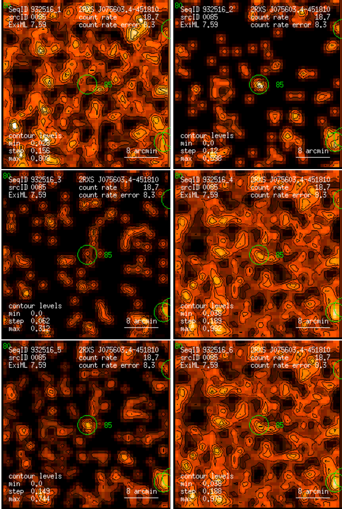
Figure 85: RASS 932516: detection 0085: band rate images, Gaussian filter: (1) PSPC channels 11 – 41, (2) 52 – 90, (3) 91 – 201, (4) 11 – 235, (5) 52 – 201, (6) 11 – 201. Broad band rates in counts/ks. Band rate contour levels in counts/ks/arcmin 2 .
