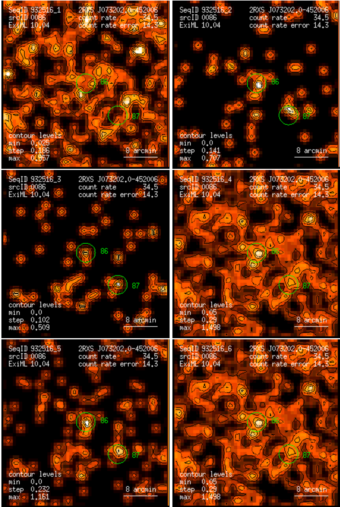
Figure 86: RASS 932516: detection 0086: band rate images, Gaussian filter: (1) PSPC channels 11 – 41, (2) 52 – 90, (3) 91 – 201, (4) 11 – 235, (5) 52 – 201, (6) 11 – 201. Broad band rates in counts/ks. Band rate contour levels in counts/ks/arcmin 2 .
