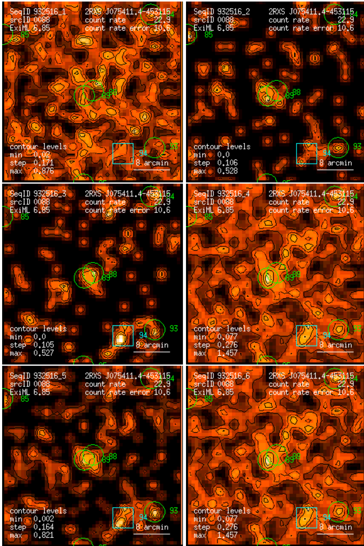
Figure 88: RASS 932516: detection 0088: band rate images, Gaussian filter: (1) PSPC channels 11 – 41, (2) 52 – 90, (3) 91 – 201, (4) 11 – 235, (5) 52 – 201, (6) 11 – 201. Broad band rates in counts/ks. Band rate contour levels in counts/ks/arcmin 2 .
