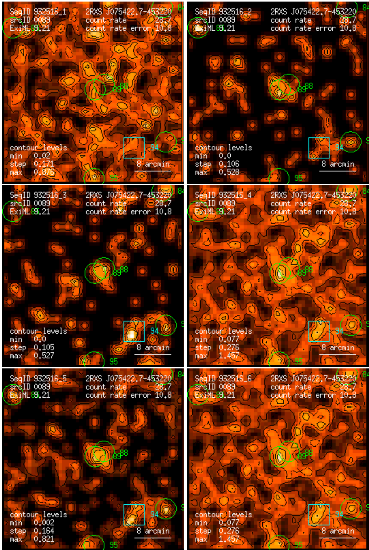
Figure 89: RASS 932516: detection 0089: band rate images, Gaussian filter: (1) PSPC channels 11 – 41, (2) 52 – 90, (3) 91 – 201, (4) 11 – 235, (5) 52 – 201, (6) 11 – 201. Broad band rates in counts/ks. Band rate contour levels in counts/ks/arcmin 2 .
