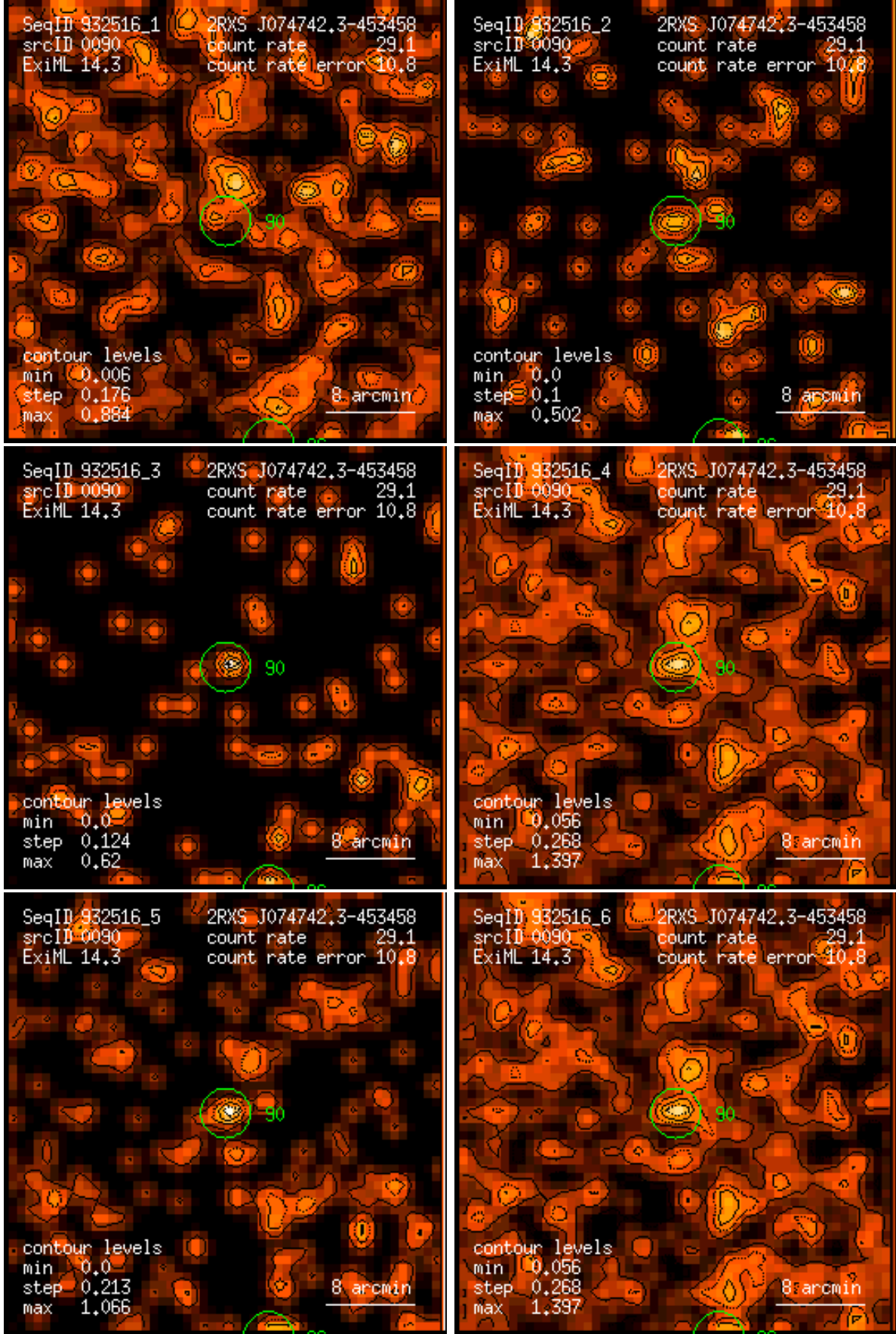
Figure 90: RASS 932516: detection 0090: band rate images, Gaussian filter: (1) PSPC channels 11 – 41, (2) 52 – 90, (3) 91 – 201, (4) 11 – 235, (5) 52 – 201, (6) 11 – 201. Broad band rates in counts/ks. Band rate contour levels in counts/ks/arcmin 2 .
