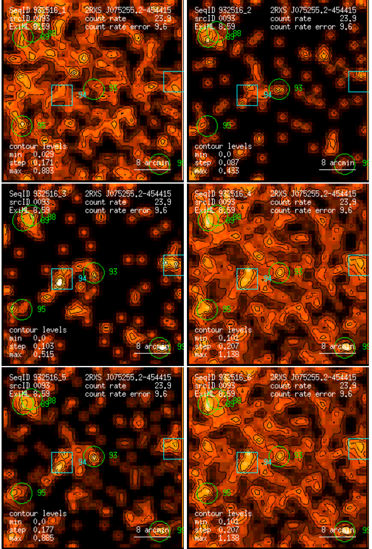
Figure 93: RASS 932516: detection 0093: band rate images, Gaussian filter: (1) PSPC channels 11 – 41, (2) 52 – 90, (3) 91 – 201, (4) 11 – 235, (5) 52 – 201, (6) 11 – 201. Broad band rates in counts/ks. Band rate contour levels in counts/ks/arcmin 2 .
