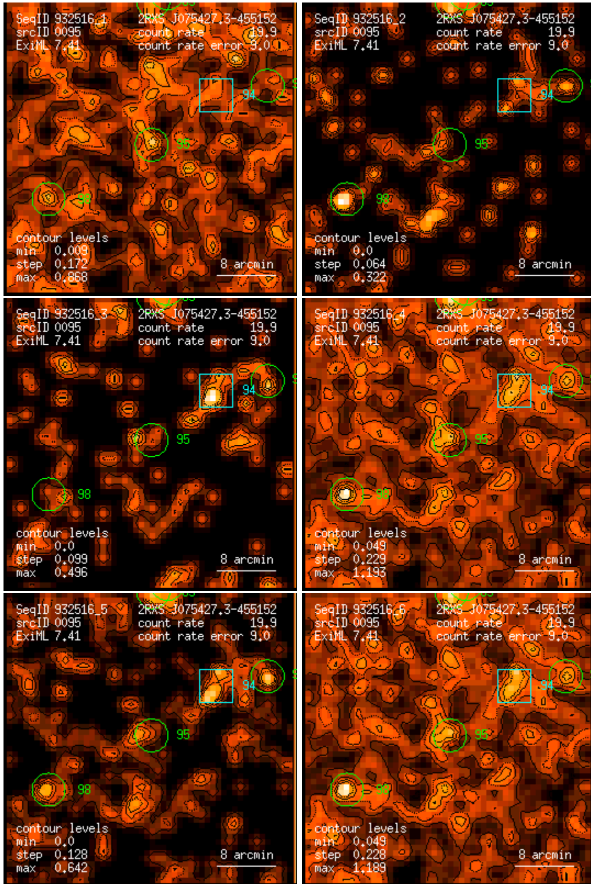
Figure 95: RASS 932516: detection 0095: band rate images, Gaussian filter: (1) PSPC channels 11 – 41, (2) 52 – 90, (3) 91 – 201, (4) 11 – 235, (5) 52 – 201, (6) 11 – 201. Broad band rates in counts/ks. Band rate contour levels in counts/ks/arcmin 2 .
