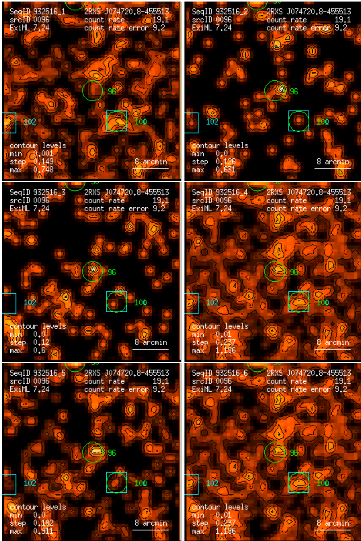
Figure 96: RASS 932516: detection 0096: band rate images, Gaussian filter: (1) PSPC channels 11 – 41, (2) 52 – 90, (3) 91 – 201, (4) 11 – 235, (5) 52 – 201, (6) 11 – 201. Broad band rates in counts/ks. Band rate contour levels in counts/ks/arcmin 2 .
