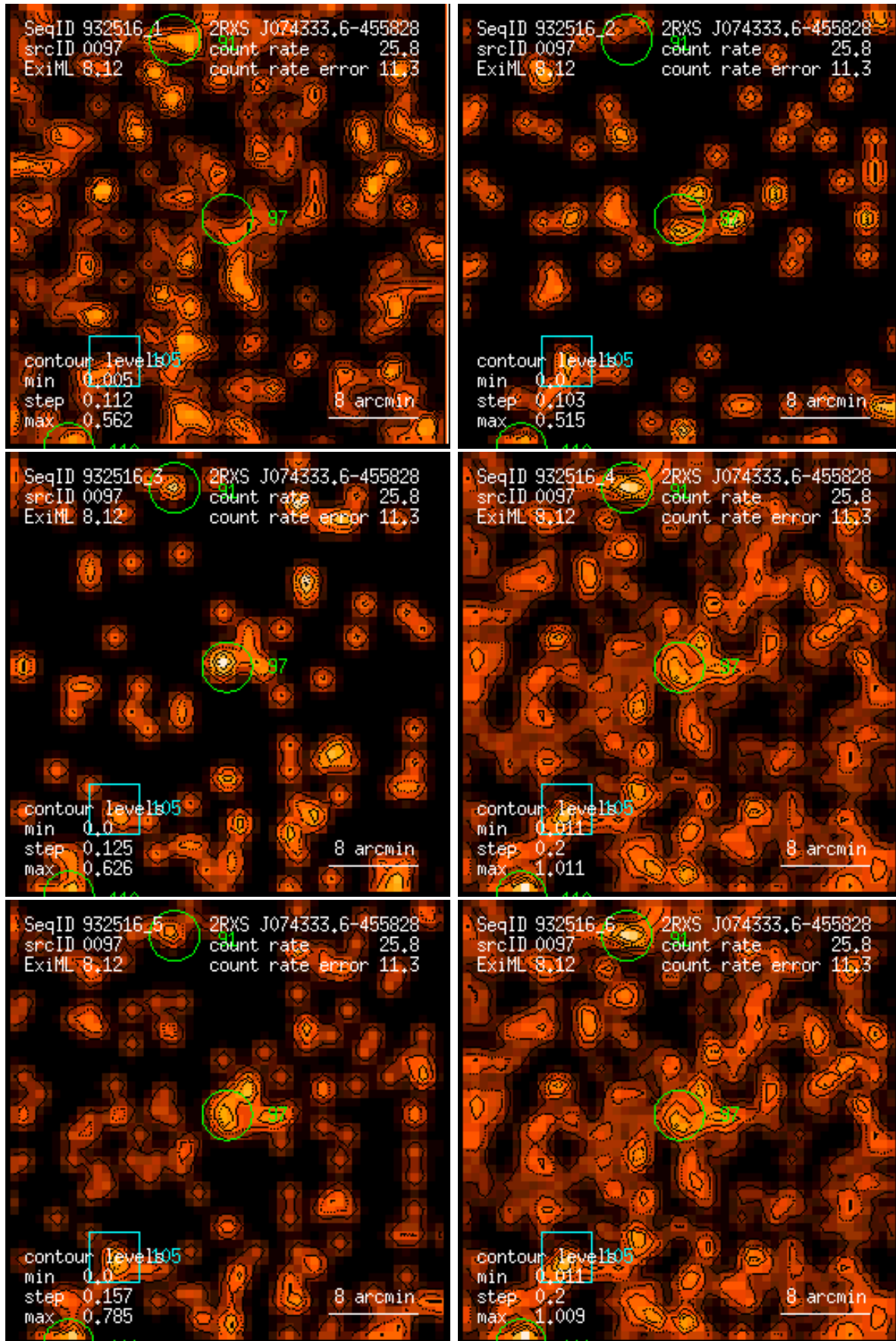
Figure 97: RASS 932516: detection 0097: band rate images, Gaussian filter: (1) PSPC channels 11 – 41, (2) 52 – 90, (3) 91 – 201, (4) 11 – 235, (5) 52 – 201, (6) 11 – 201. Broad band rates in counts/ks. Band rate contour levels in counts/ks/arcmin 2 .
