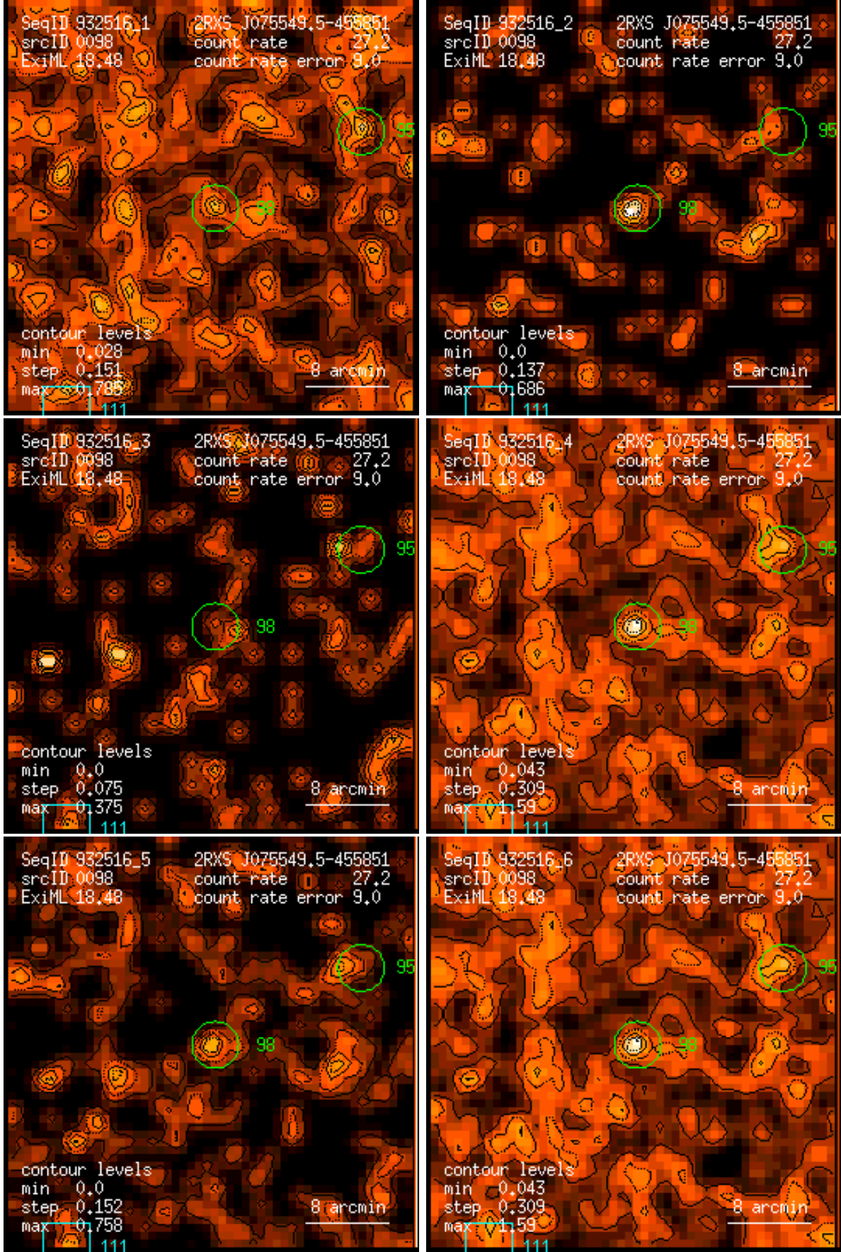
Figure 98: RASS 932516: detection 0098: band rate images, Gaussian filter: (1) PSPC channels 11 – 41, (2) 52 – 90, (3) 91 – 201, (4) 11 – 235, (5) 52 – 201, (6) 11 – 201. Broad band rates in counts/ks. Band rate contour levels in counts/ks/arcmin 2 .
