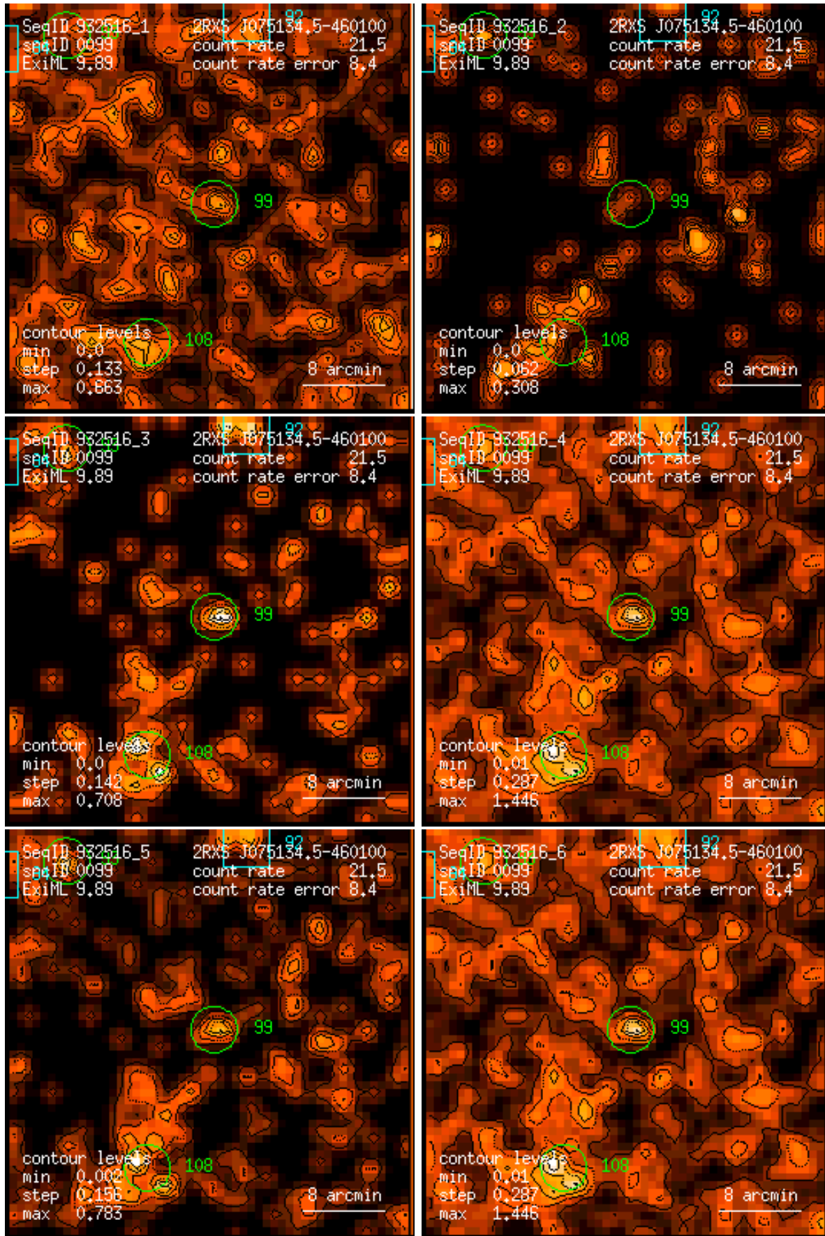
Figure 99: RASS 932516: detection 0099: band rate images, Gaussian filter: (1) PSPC channels 11 – 41, (2) 52 – 90, (3) 91 – 201, (4) 11 – 235, (5) 52 – 201, (6) 11 – 201. Broad band rates in counts/ks. Band rate contour levels in counts/ks/arcmin 2 .
