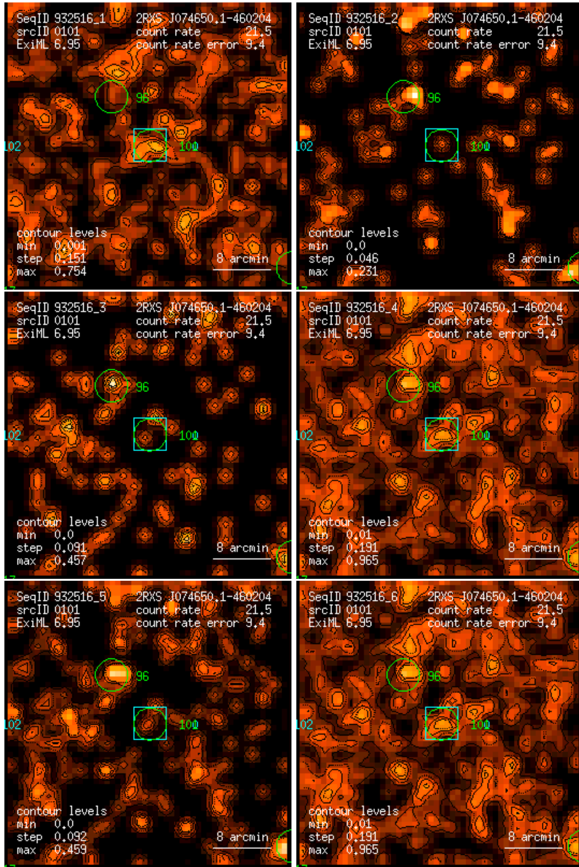
Figure 101: RASS 932516: detection 0101: band rate images, Gaussian filter: (1) PSPC channels 11 – 41, (2) 52 – 90, (3) 91 – 201, (4) 11 – 235, (5) 52 – 201, (6) 11 – 201. Broad band rates in counts/ks. Band rate contour levels in counts/ks/arcmin 2 .
