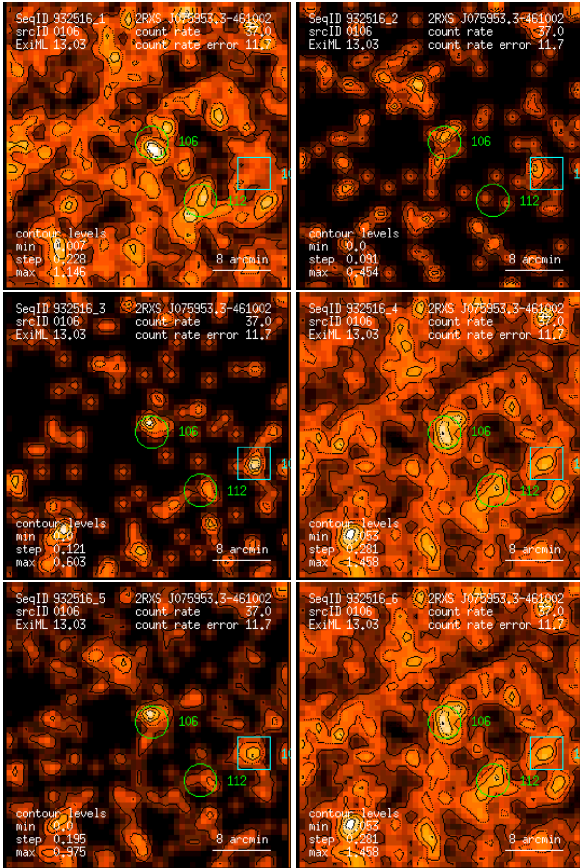
Figure 106: RASS 932516: detection 0106: band rate images, Gaussian filter: (1) PSPC channels 11 – 41, (2) 52 – 90, (3) 91 – 201, (4) 11 – 235, (5) 52 – 201, (6) 11 – 201. Broad band rates in counts/ks. Band rate contour levels in counts/ks/arcmin 2 .
