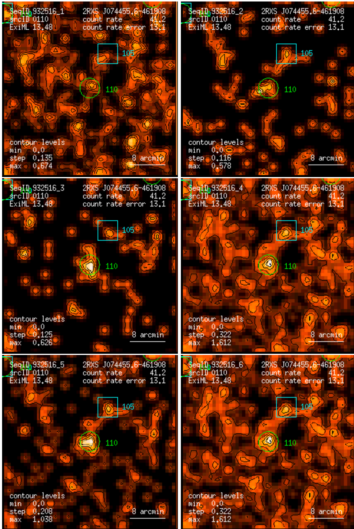
Figure 110: RASS 932516: detection 0110: band rate images, Gaussian filter: (1) PSPC channels 11 – 41, (2) 52 – 90, (3) 91 – 201, (4) 11 – 235, (5) 52 – 201, (6) 11 – 201. Broad band rates in counts/ks. Band rate contour levels in counts/ks/arcmin 2 .
