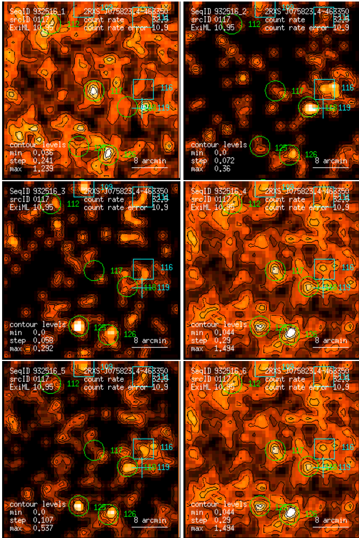
Figure 117: RASS 932516: detection 0117: band rate images, Gaussian filter: (1) PSPC channels 11 – 41, (2) 52 – 90, (3) 91 – 201, (4) 11 – 235, (5) 52 – 201, (6) 11 – 201. Broad band rates in counts/ks. Band rate contour levels in counts/ks/arcmin 2 .
