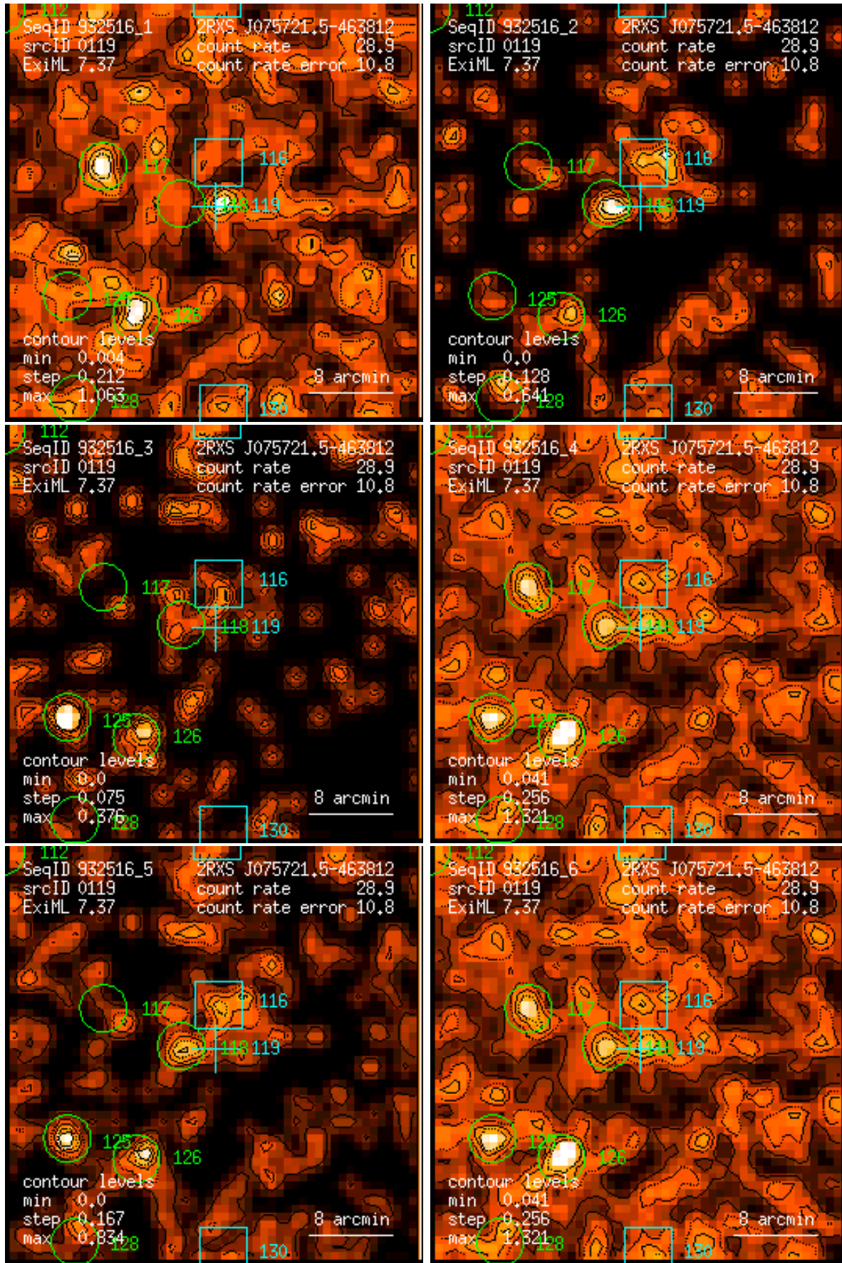
Figure 119: RASS 932516: detection 0119: band rate images, Gaussian filter: (1) PSPC channels 11 – 41, (2) 52 – 90, (3) 91 – 201, (4) 11 – 235, (5) 52 – 201, (6) 11 – 201. Broad band rates in counts/ks. Band rate contour levels in counts/ks/arcmin 2 .
