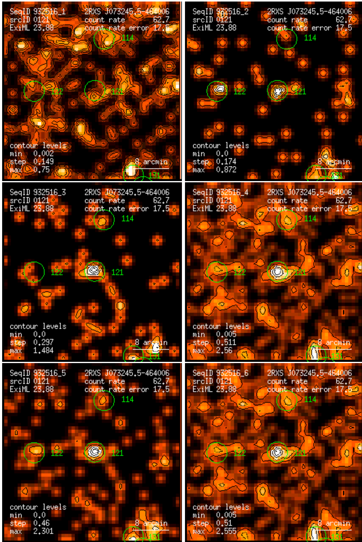
Figure 121: RASS 932516: detection 0121: band rate images, Gaussian filter: (1) PSPC channels 11 – 41, (2) 52 – 90, (3) 91 – 201, (4) 11 – 235, (5) 52 – 201, (6) 11 – 201. Broad band rates in counts/ks. Band rate contour levels in counts/ks/arcmin 2 .
