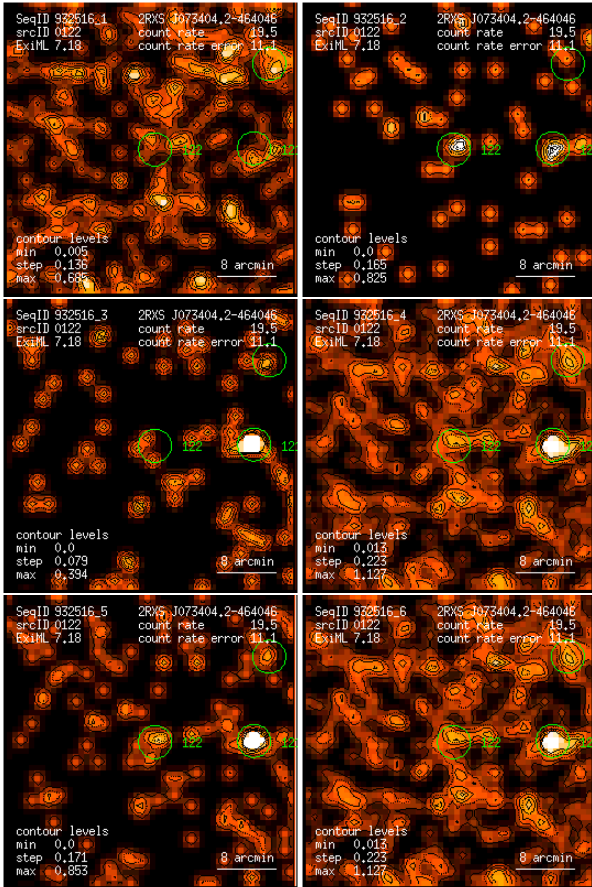
Figure 122: RASS 932516: detection 0122: band rate images, Gaussian filter: (1) PSPC channels 11 – 41, (2) 52 – 90, (3) 91 – 201, (4) 11 – 235, (5) 52 – 201, (6) 11 – 201. Broad band rates in counts/ks. Band rate contour levels in counts/ks/arcmin 2 .
