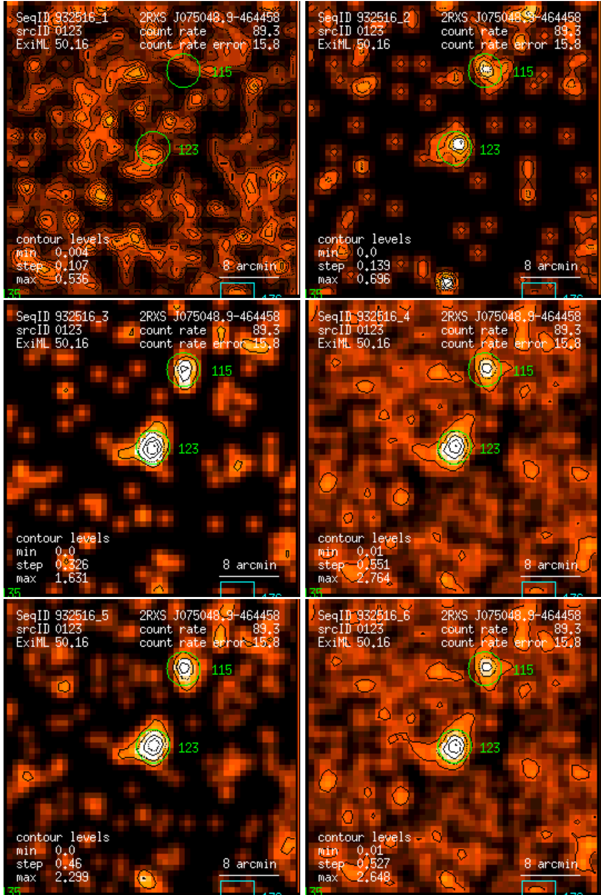
Figure 123: RASS 932516: detection 0123: band rate images, Gaussian filter: (1) PSPC channels 11 – 41, (2) 52 – 90, (3) 91 – 201, (4) 11 – 235, (5) 52 – 201, (6) 11 – 201. Broad band rates in counts/ks. Band rate contour levels in counts/ks/arcmin 2 .
