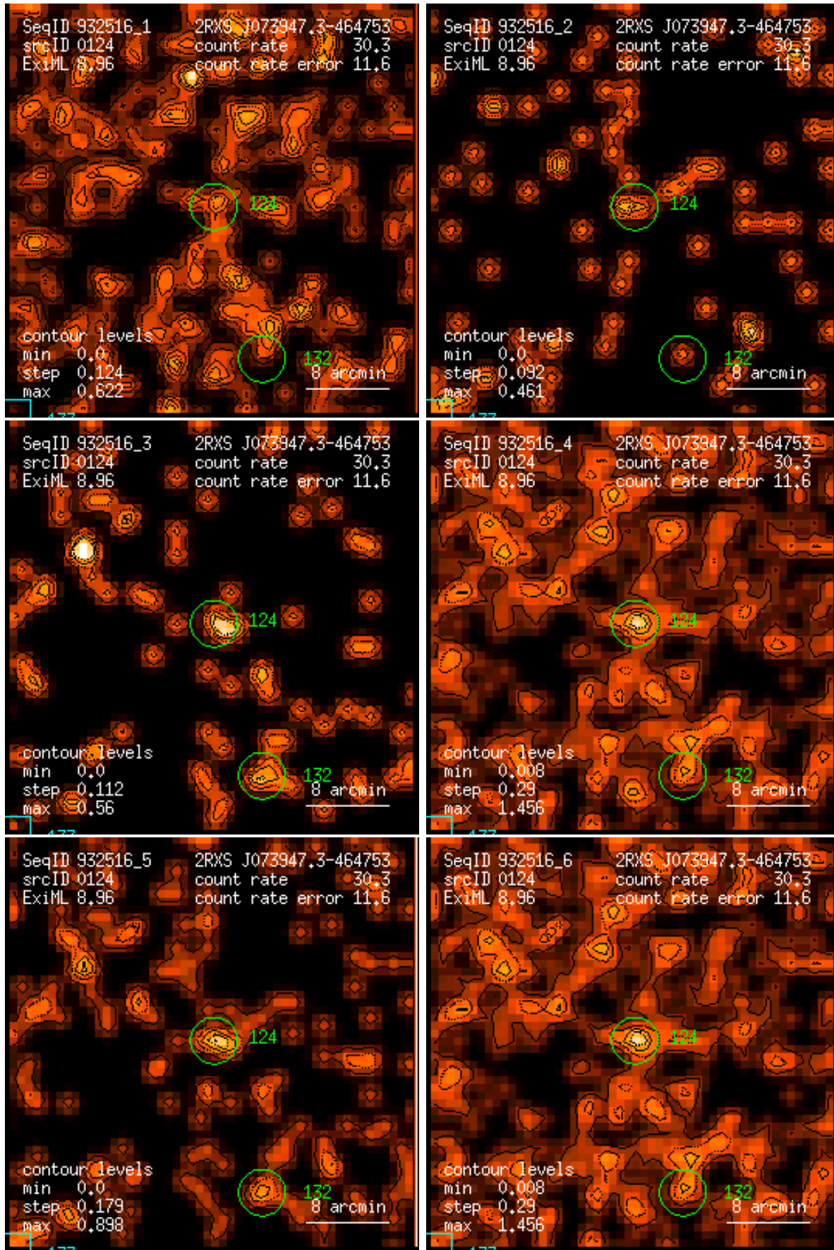
Figure 124: RASS 932516: detection 0124: band rate images, Gaussian filter: (1) PSPC channels 11 – 41, (2) 52 – 90, (3) 91 – 201, (4) 11 – 235, (5) 52 – 201, (6) 11 – 201. Broad band rates in counts/ks. Band rate contour levels in counts/ks/arcmin 2 .
