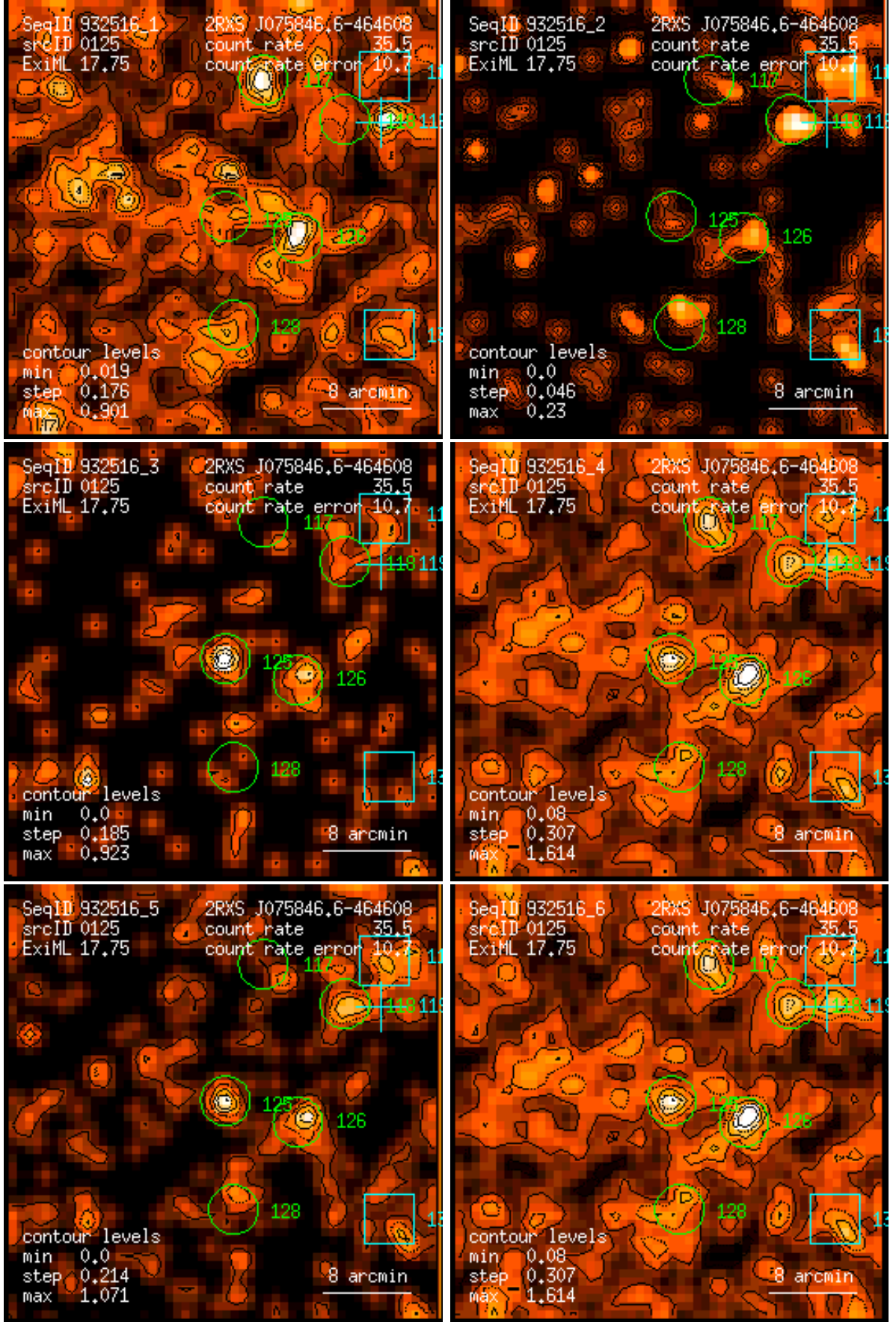
Figure 125: RASS 932516: detection 0125: band rate images, Gaussian filter: (1) PSPC channels 11 – 41, (2) 52 – 90, (3) 91 – 201, (4) 11 – 235, (5) 52 – 201, (6) 11 – 201. Broad band rates in counts/ks. Band rate contour levels in counts/ks/arcmin 2 .
